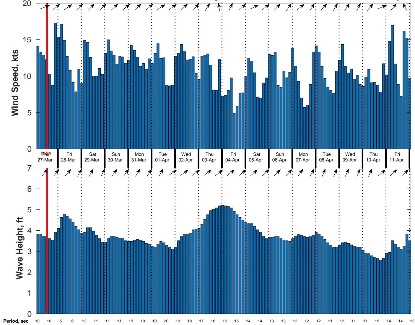
Wind & Wave Forecast for CSA (ONHYM) PPL EBS - Nigeria from 26-Mar-2025 02:00:00 to 11-Apr-2025 02:00:00
