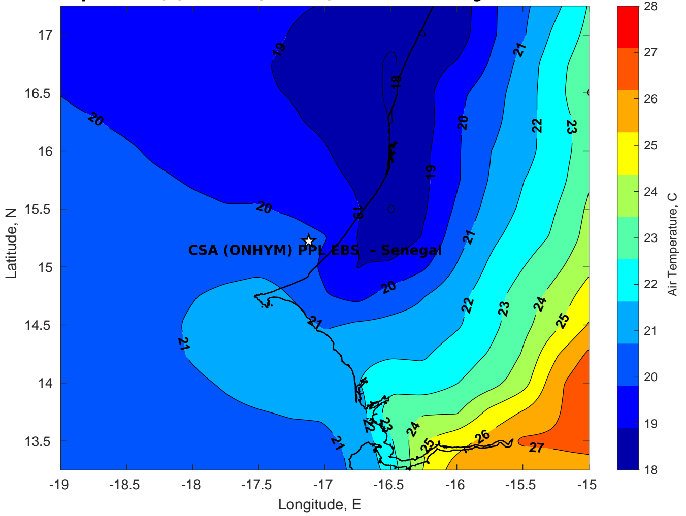
Air Temperature (C) for CSA (ONHYM) PPL EBS - Senegal at 26-Mar-2025
