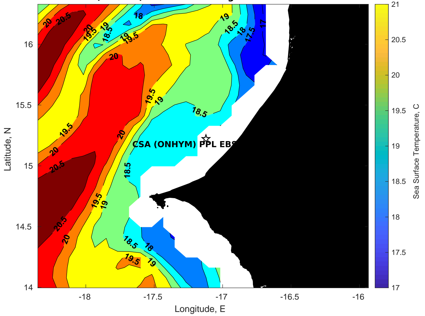
SST for CSA (ONHYM) PPL EBS - Senegal at 25-Mar-2025 00:00:00
