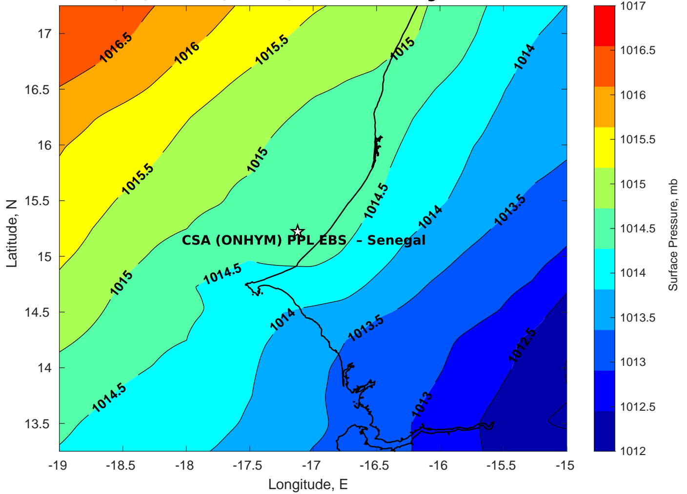
Surface Pressure (mb) for CSA (ONHYM) PPL EBS - Senegal at 26-Mar-2025 00:00:00
