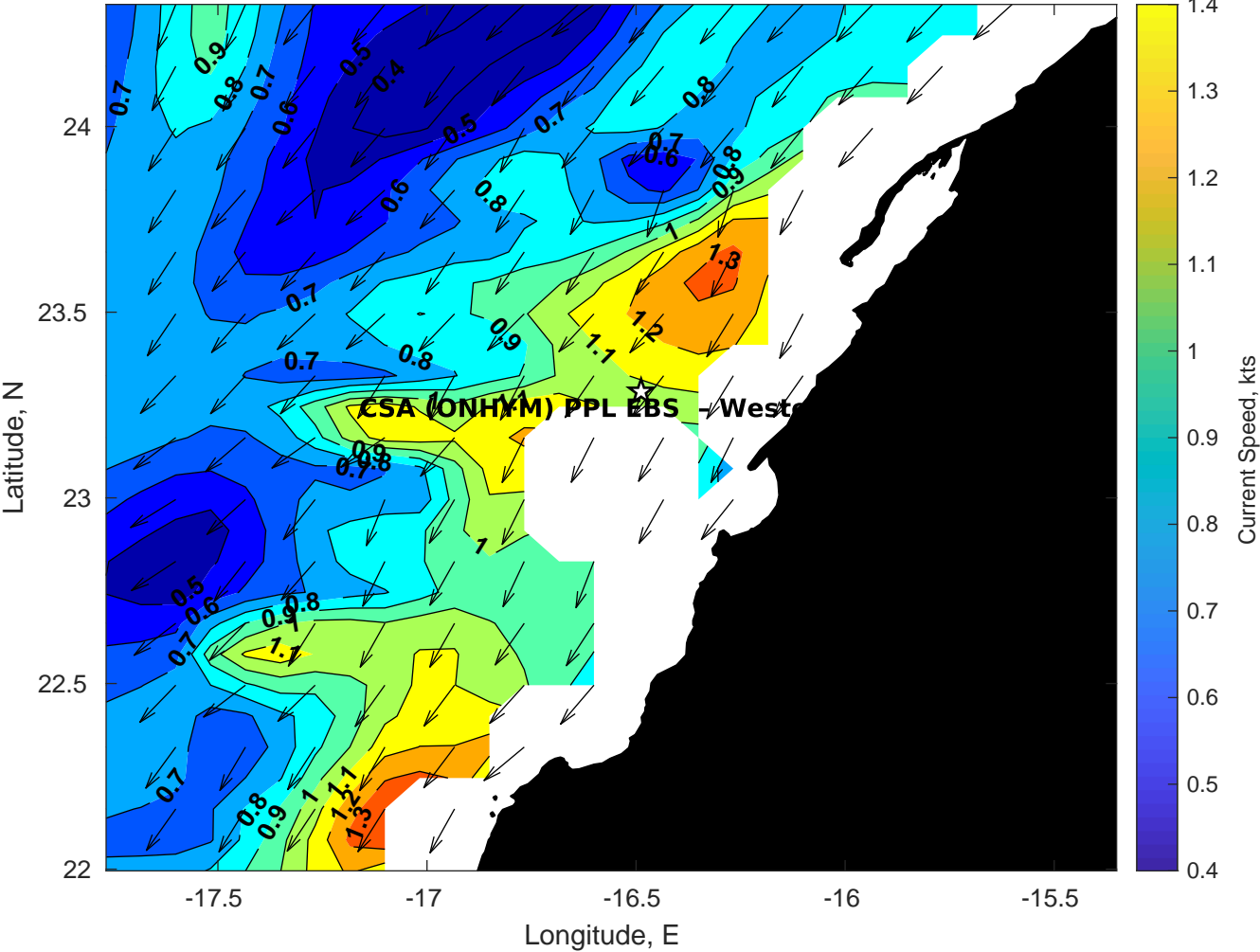
Surface Currents for CSA (ONHYM) PPL EBS - Western Sahara at 25-Mar-2025 00:00:00
