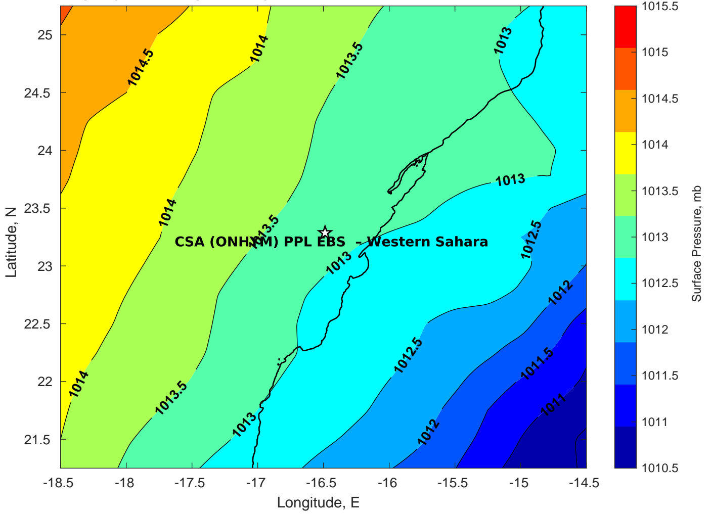
Surface Pressure (mb) for CSA (ONHYM) PPL EBS - Western Sahara at 28-Mar-2025 00:00:00
