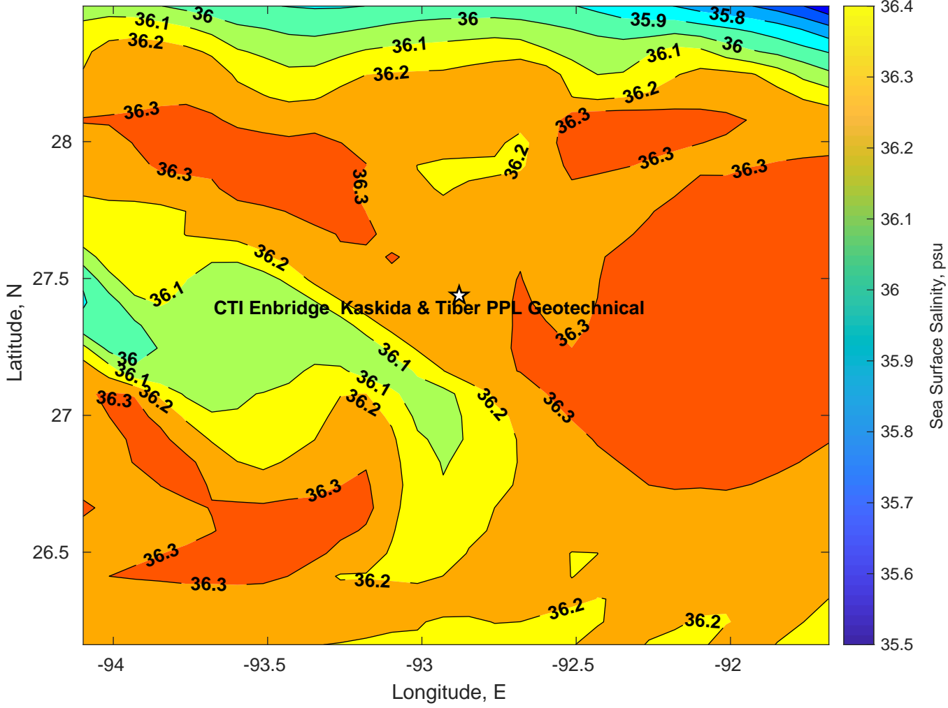
Surface Salinity for CTI Enbridge Kaskida & Tiber PPL Geotechnical at 25-Mar-2025 00:00:00
