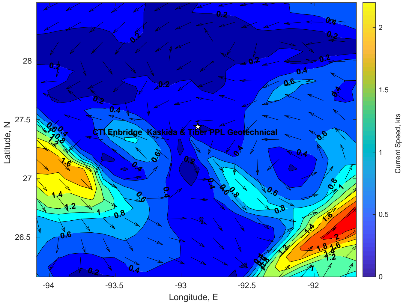
Surface Currents for CTI Enbridge Kaskida & Tiber PPL Geotechnical at 25-Mar-2025 00:00:00
