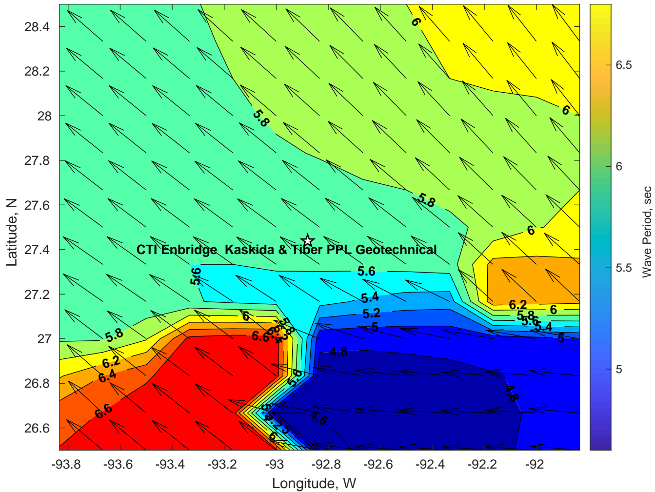
Wave Period (sec) for CTI Enbridge Kaskida & Tiber PPL Geotechnical at 26-Mar-2025 09:00:00
