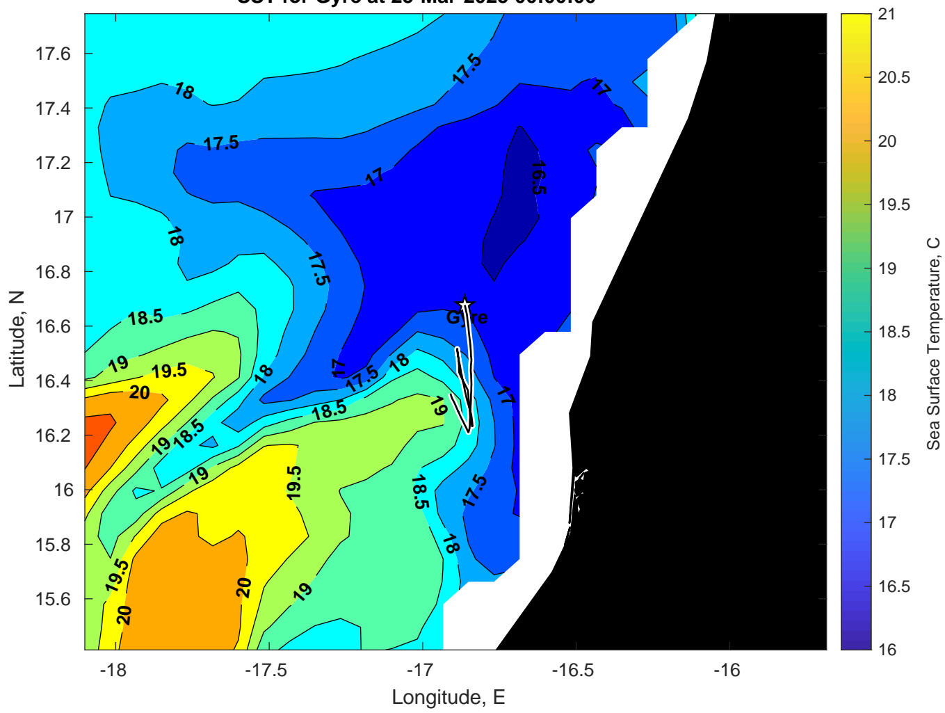
SST for Gyre at 25-Mar-2025 00:00:00
