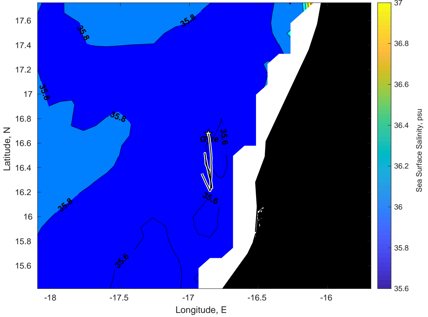
Surface Salinity for Gyre at 25-Mar-2025 00:00:00
