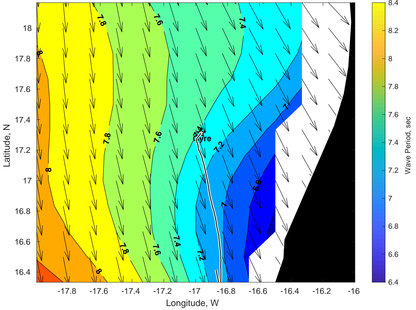
Wave Period (sec) for Gyre at 26-Mar-2025 09:00:00
