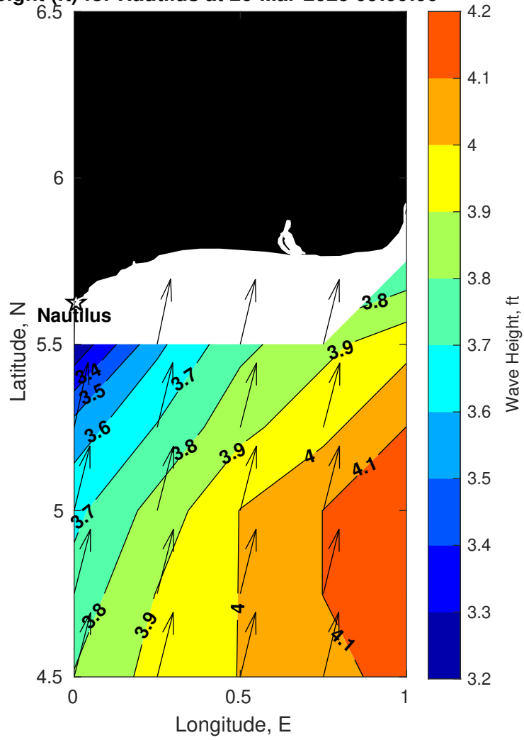
Wave Height (ft) for Nautilus at 26-Mar-2025 09:00:00
