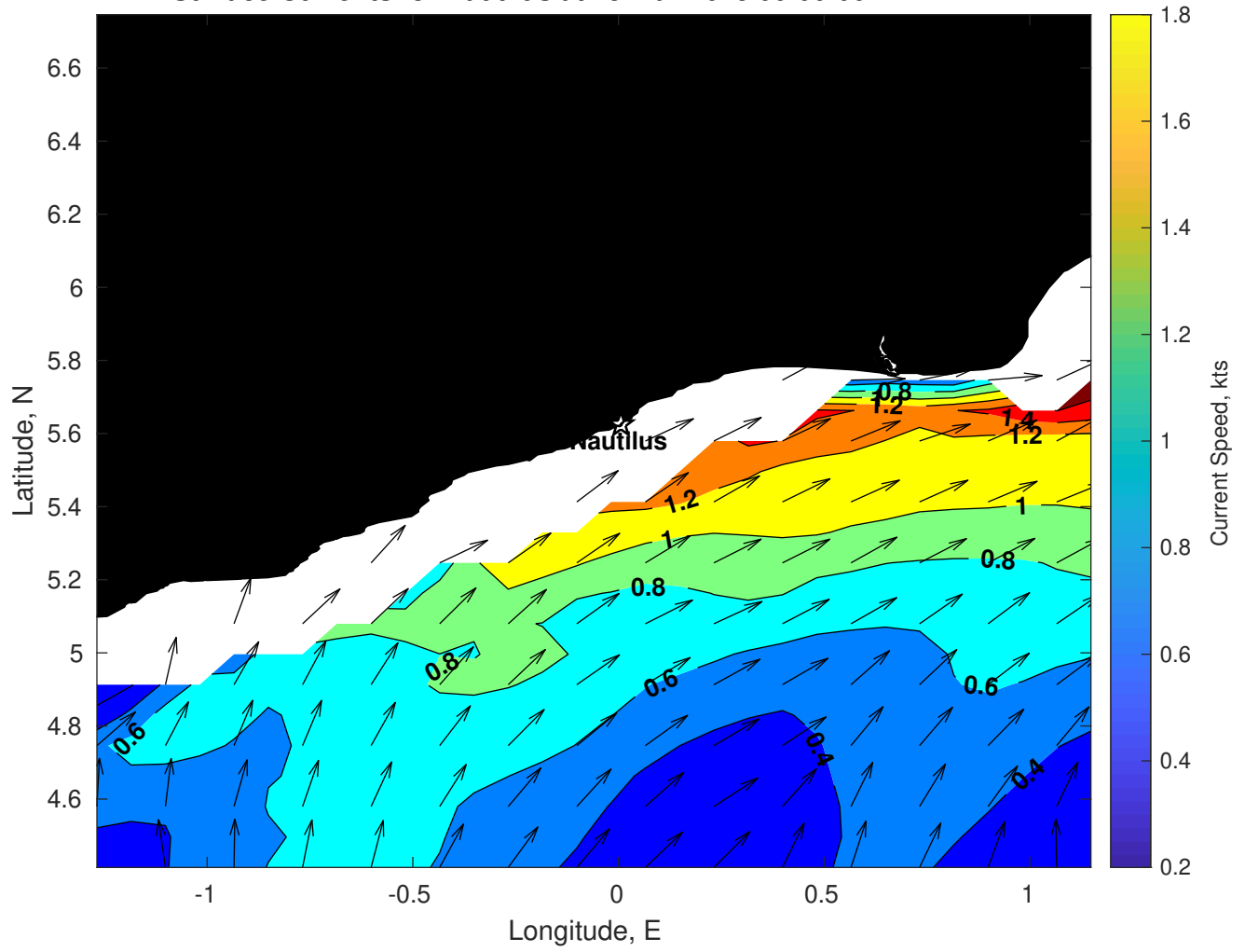
Surface Currents for Nautilus at 25-Mar-2025 00:00:00
