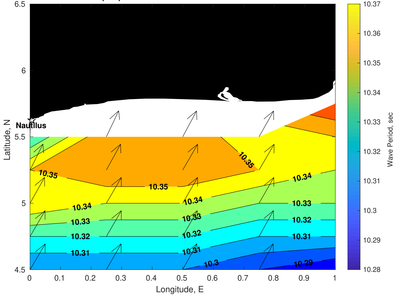
Wave Period (sec) for Nautilus at 26-Mar-2025 09:00:00
