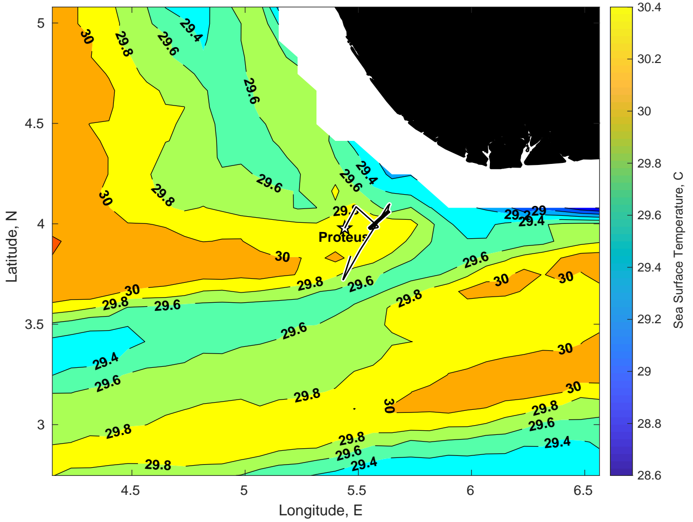
SST for Proteus at 25-Mar-2025 00:00:00
