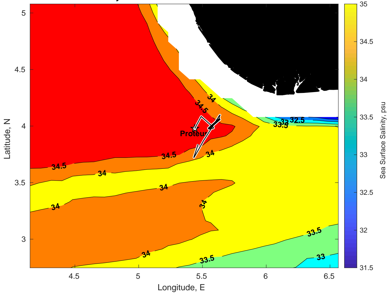
Surface Salinity for Proteus at 25-Mar-2025 00:00:00
