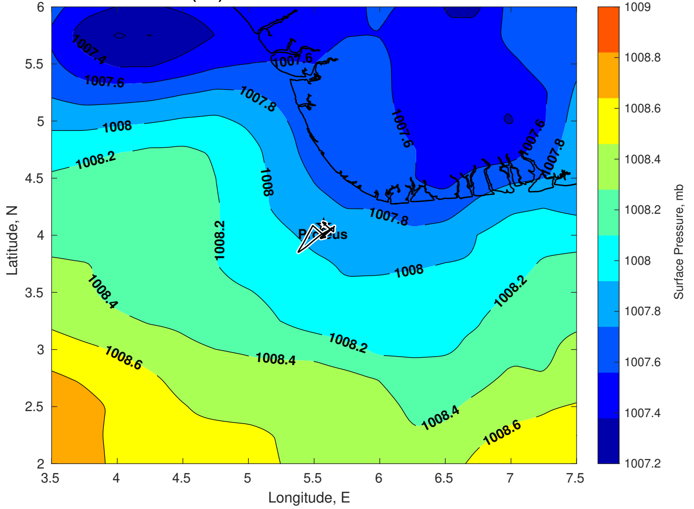
Surface Pressure (mb) for Proteus at 28-Mar-2025 00:00:00
