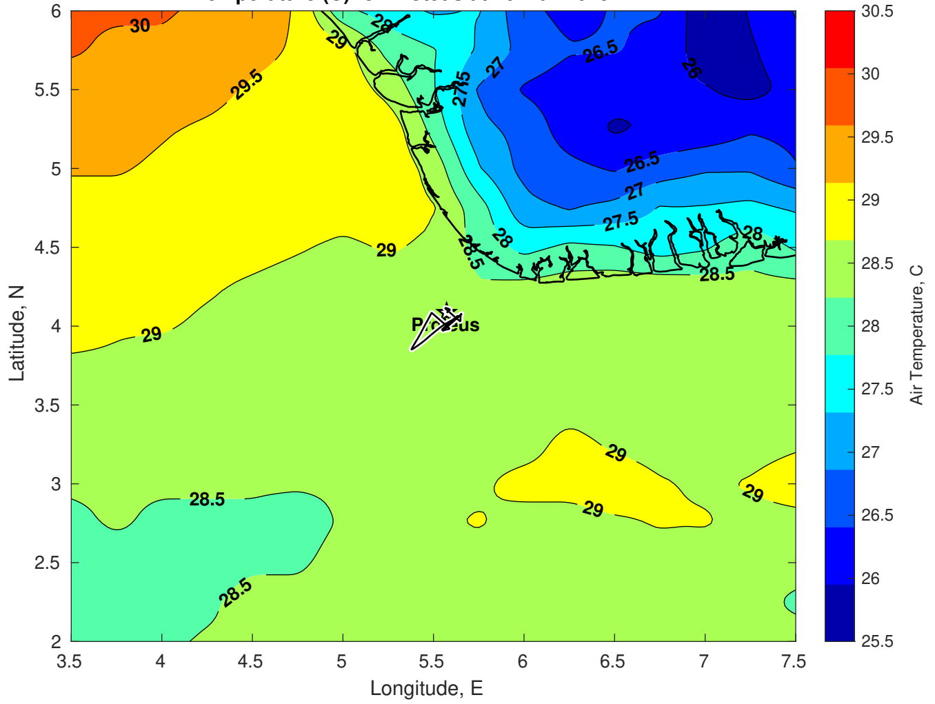
Air Temperature (C) for Proteus at 26-Mar-2025
