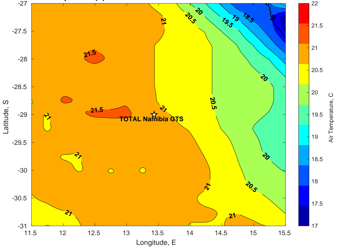
Air Temperature (C) for TOTAL Namibia GTS at 26-Mar-2025
