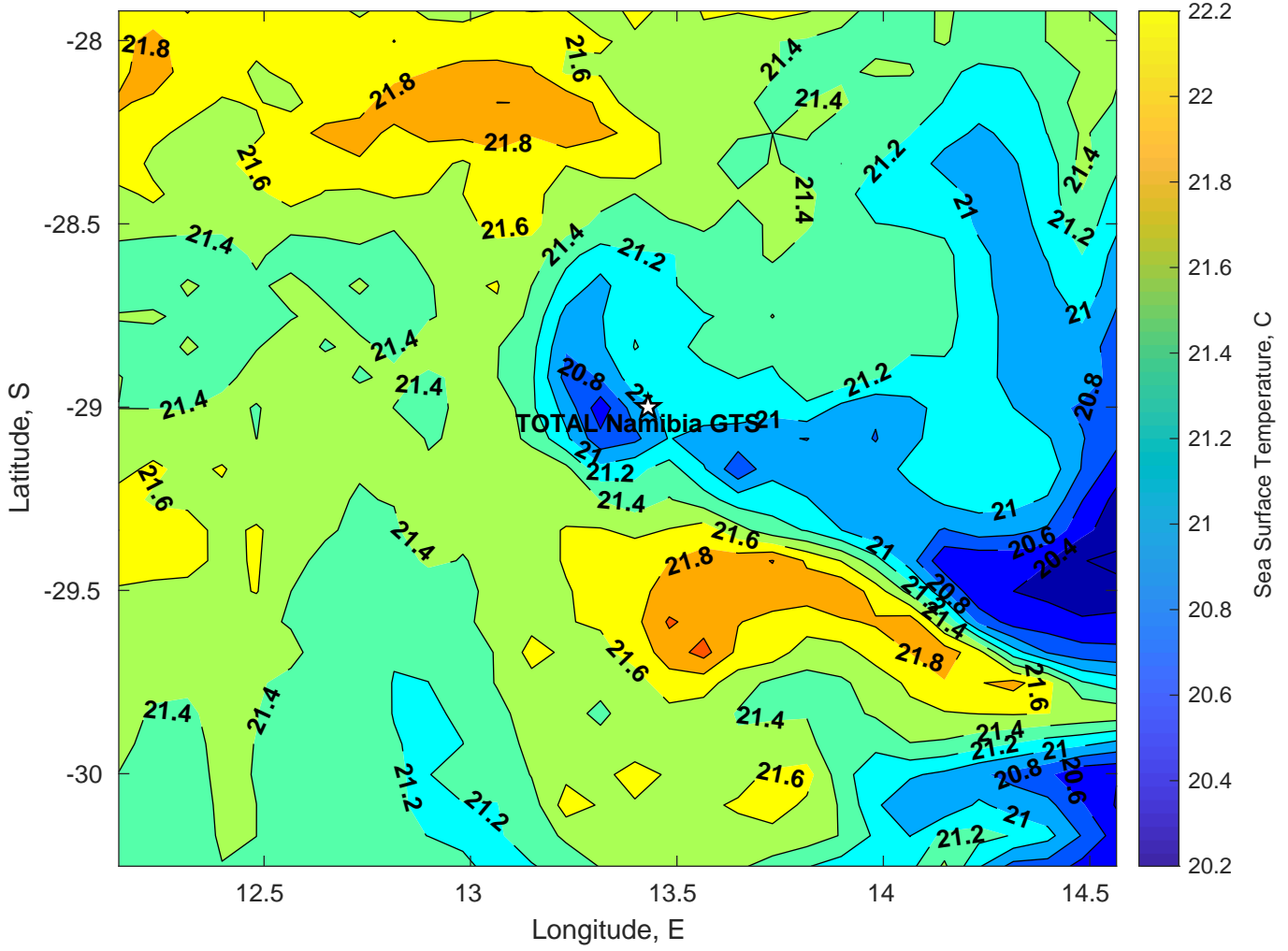
SST for TOTAL Namibia GTS at 25-Mar-2025 00:00:00
