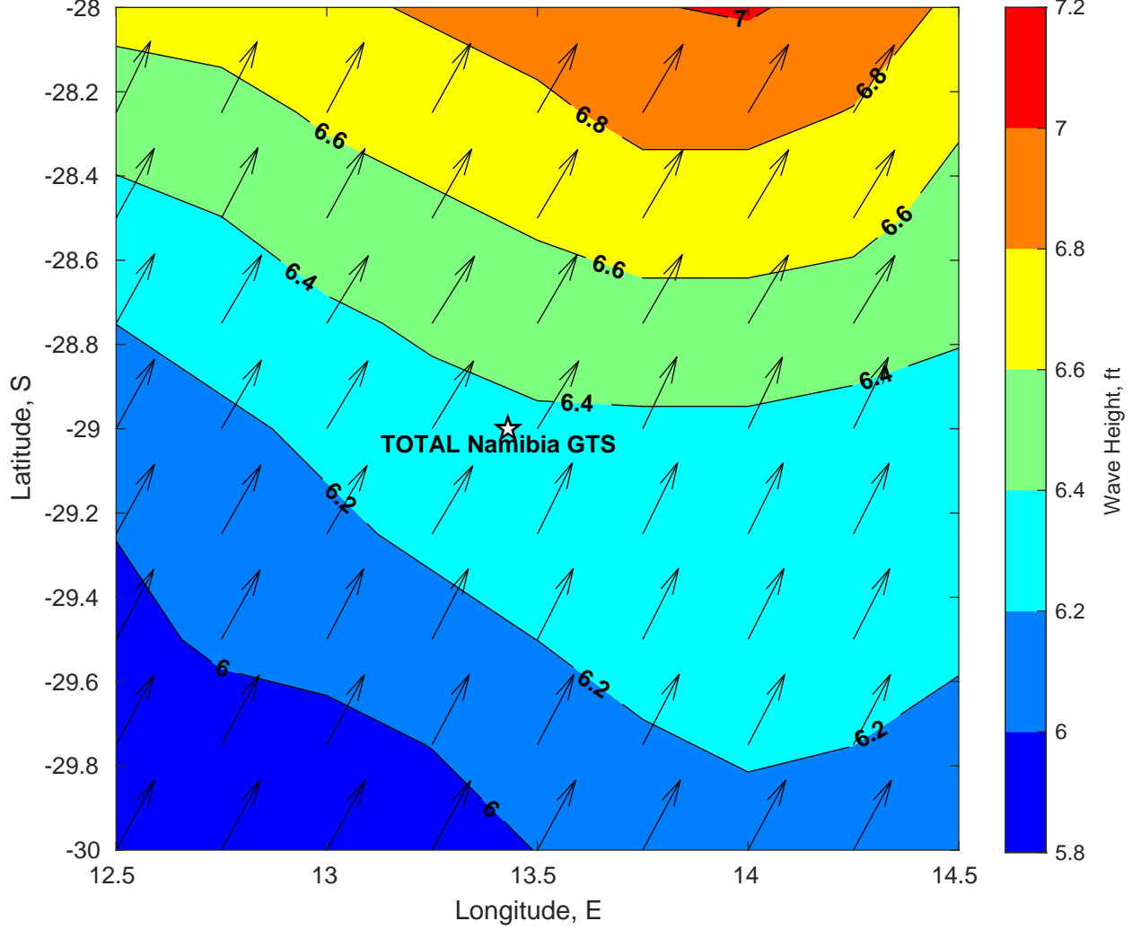
Wave Height (ft) for TOTAL Namibia GTS at 26-Mar-2025 09:00:00
