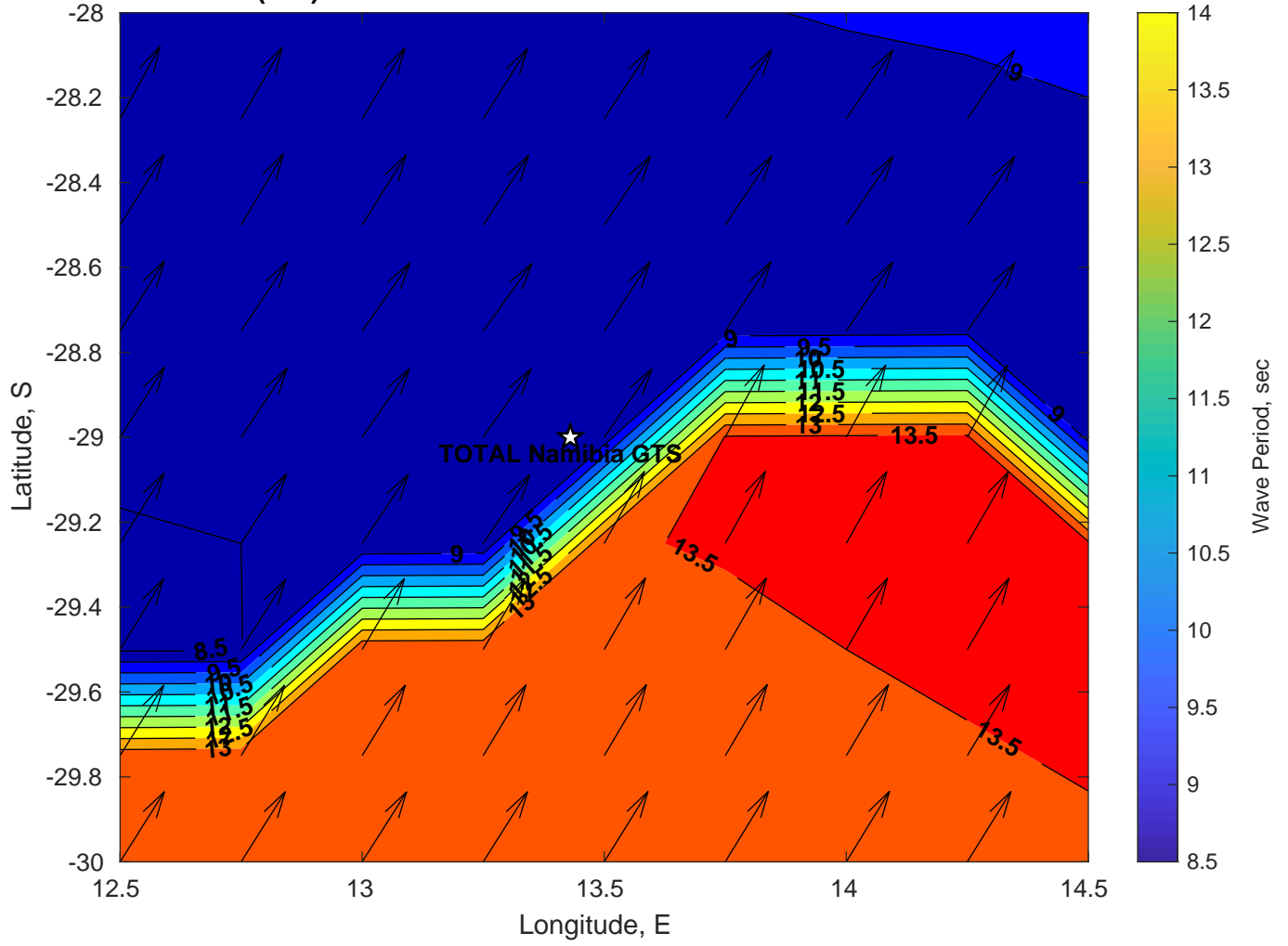
Wave Period (sec) for TOTAL Namibia GTS at 26-Mar-2025 09:00:00
