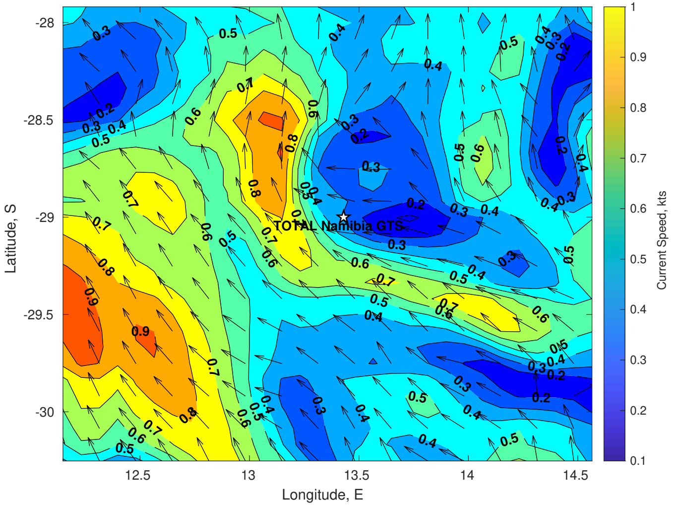
Surface Currents for TOTAL Namibia GTS at 25-Mar-2025 00:00:00
