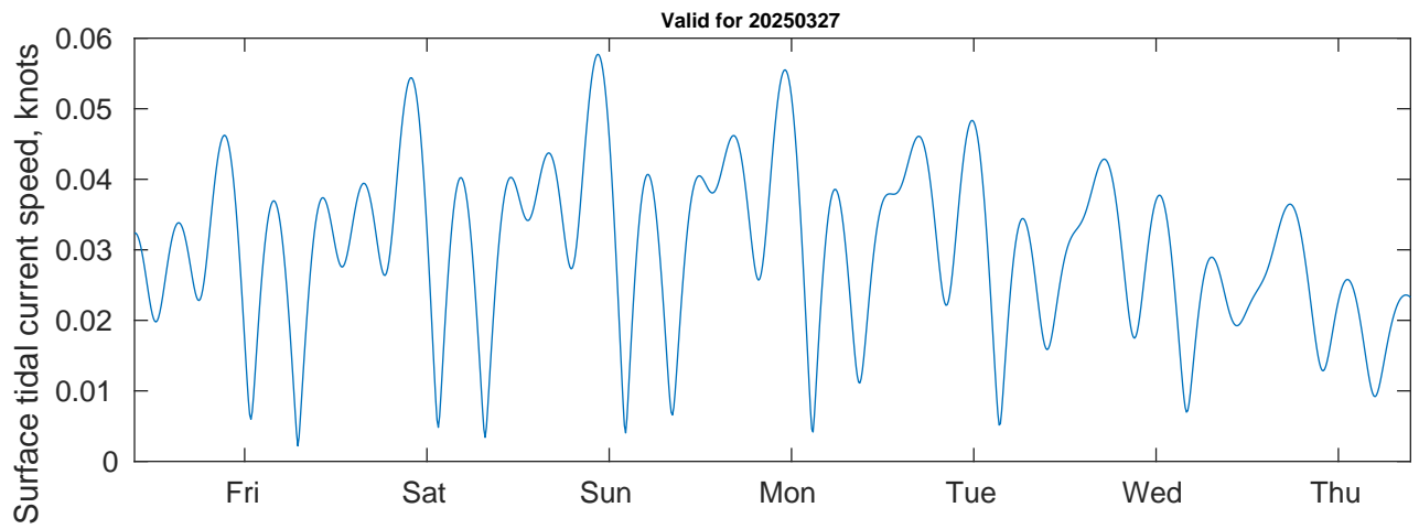
Tidal Currents and Heights for Benthic Solutions South Africa HF Site1 at 20250327
