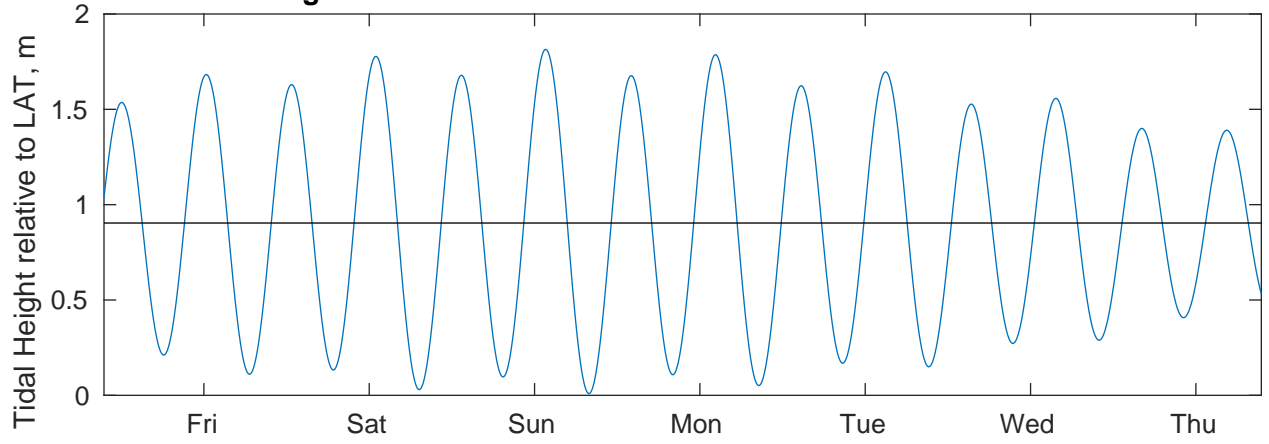
Tidal Currents and Heights for Benthic Solutions South Africa HF Site1 at 20250327
