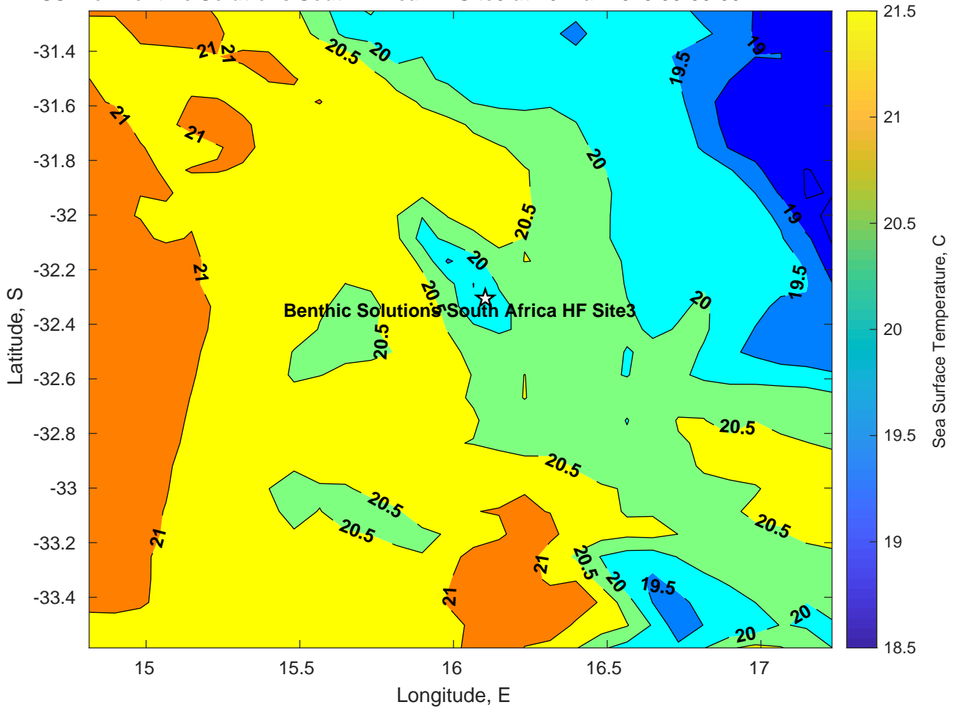
SST for Benthic Solutions South Africa HF Site3 at 26-Mar-2025 00:00:00
