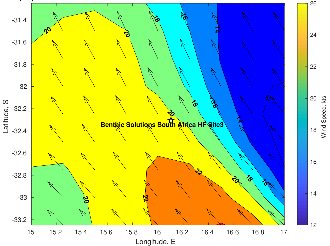
Winds (kts) for Benthic Solutions South Africa HF Site3 at 27-Mar-2025 09:00:00
