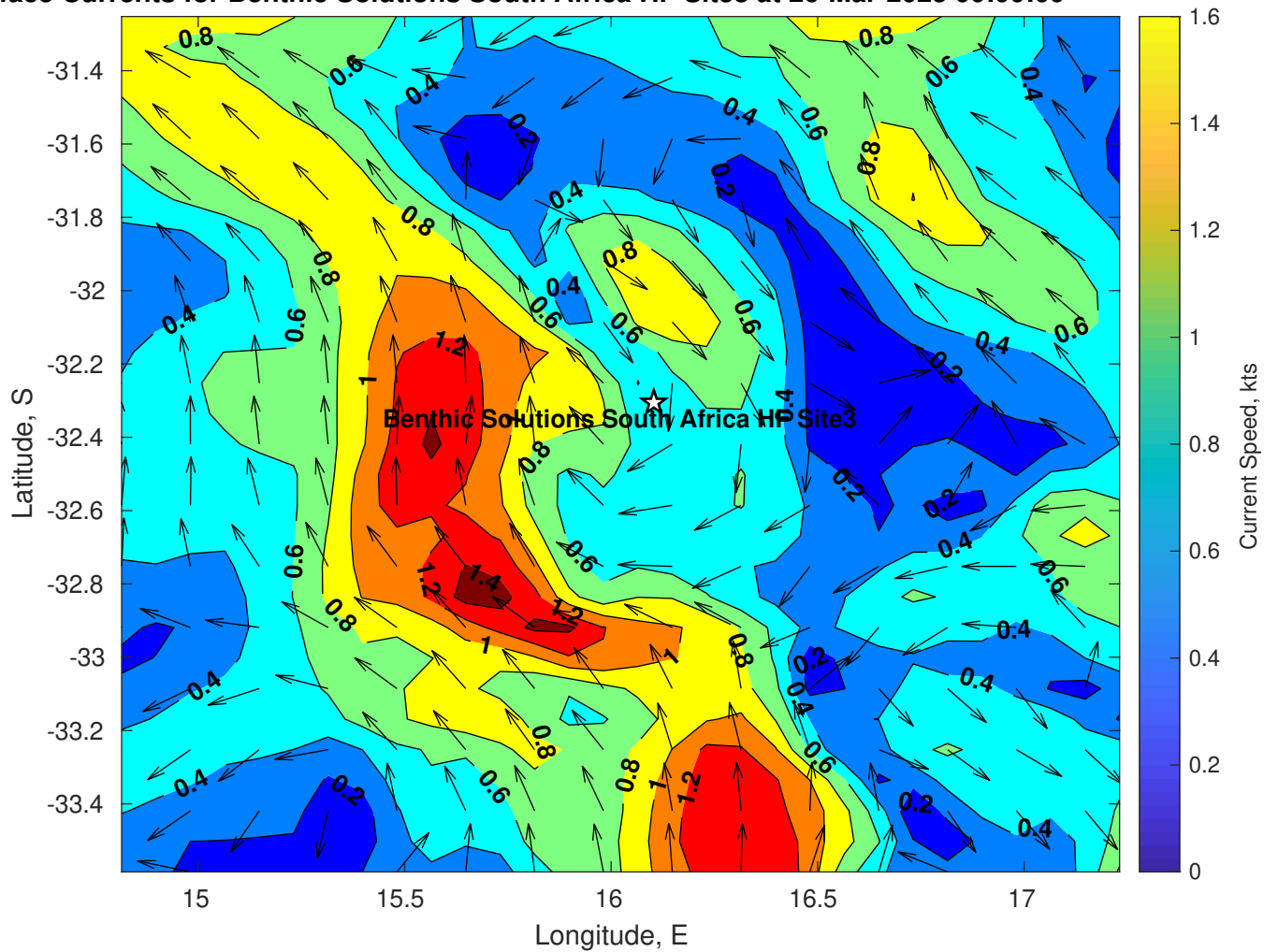
Surface Currents for Benthic Solutions South Africa HF Site3 at 26-Mar-2025 00:00:00
