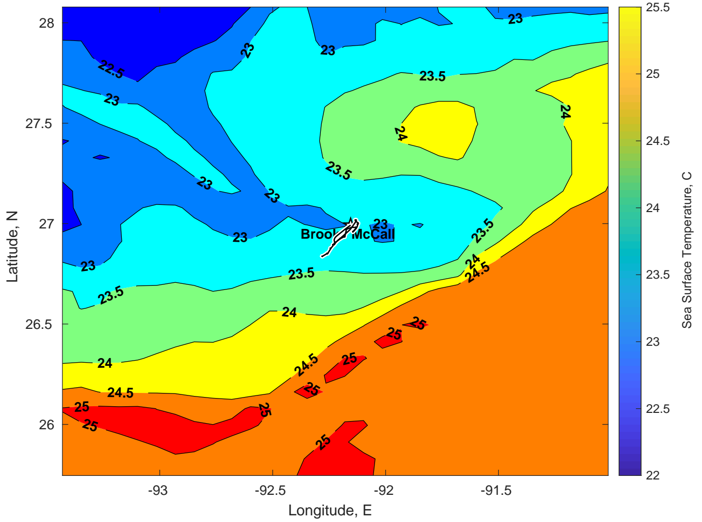
SST for Brooks McCall at 26-Mar-2025 00:00:00
