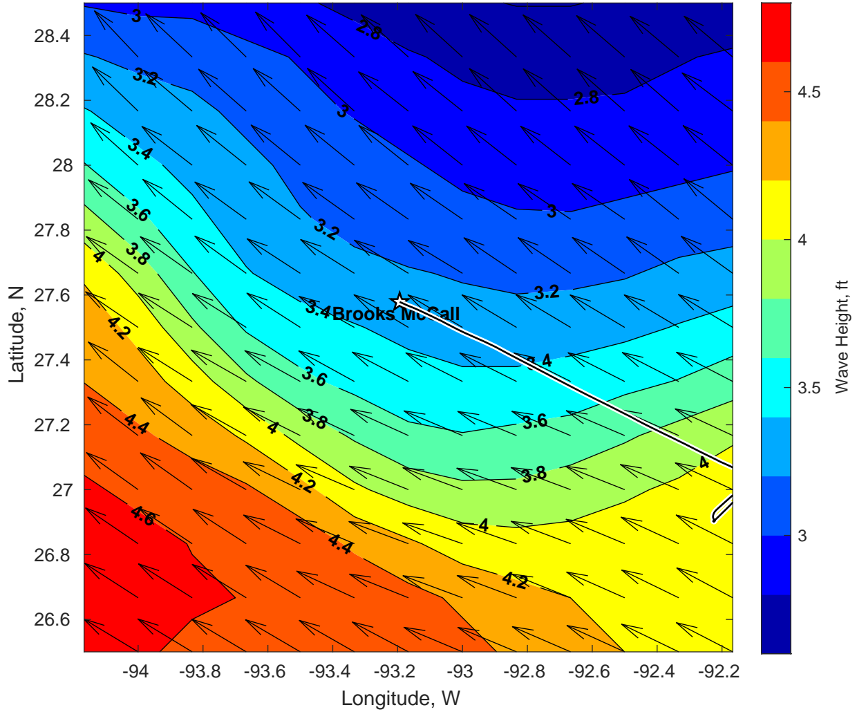
Wave Height (ft) for Brooks McCall at 27-Mar-2025 09:00:00
