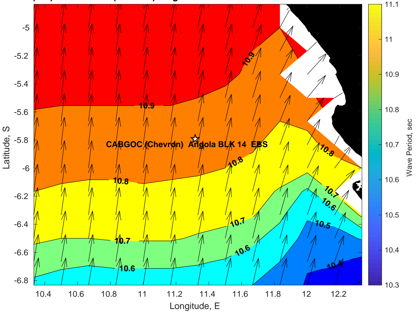
Wave Period (sec) for CABGOC (Chevron) Angola BLK 14 EBS at 27-Mar-2025 09:00:00
