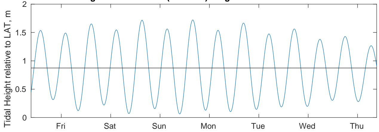
Tidal Currents and Heights for CABGOC (Chevron) Angola BLK 14 EBS at 20250327
