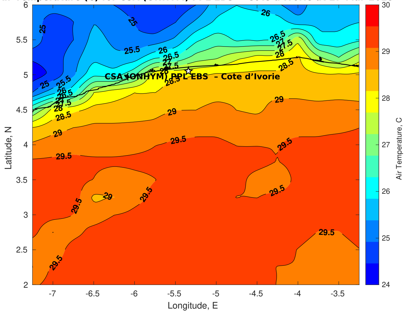
Air Temperature (C) for CSA (ONHYM) PPL EBS - Cote d'Ivoire at 27-Mar-2025
