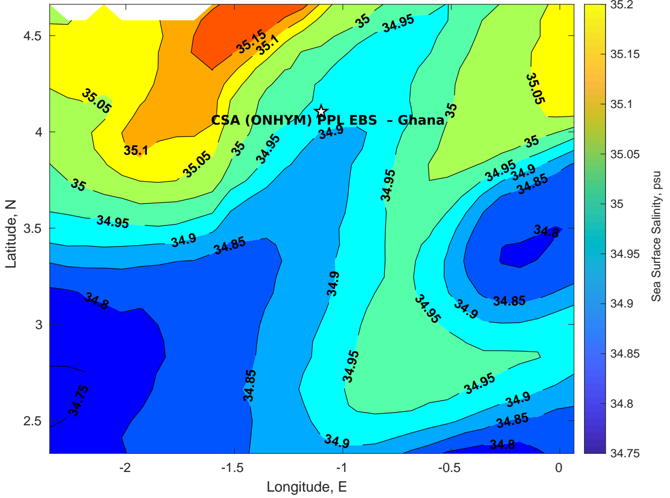
Surface Salinity for CSA (ONHYM) PPL EBS - Ghana at 26-Mar-2025 00:00:00
