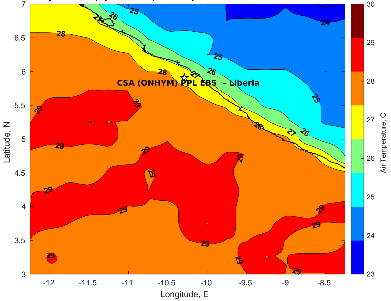
Air Temperature (C) for CSA (ONHYM) PPL EBS - Liberia at 27-Mar-2025
