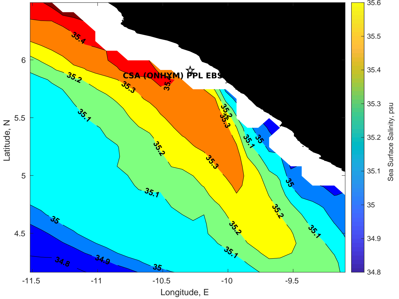
Surface Salinity for CSA (ONHYM) PPL EBS - Liberia at 26-Mar-2025 00:00:00
