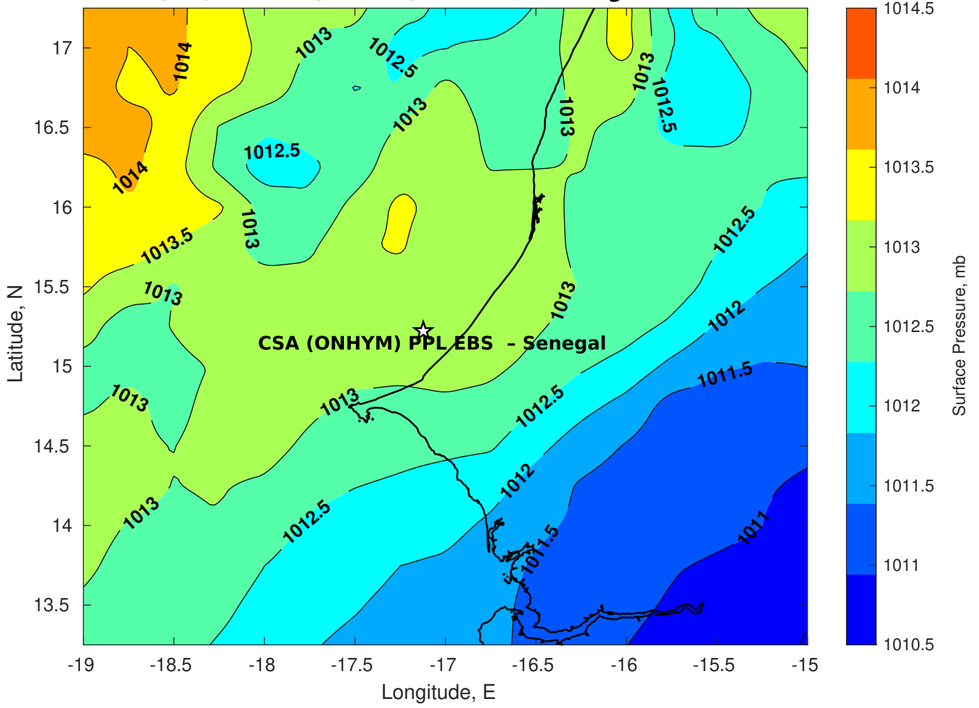
Surface Pressure (mb) for CSA (ONHYM) PPL EBS - Senegal at 29-Mar-2025 00:00:00
