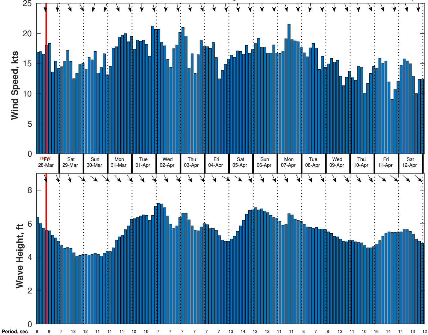
Wind & Wave Forecast for CSA (ONHYM) PPL EBS - Senegal from 27-Mar-2025 01:00:00 to 12-Apr-2025 01:00:00
