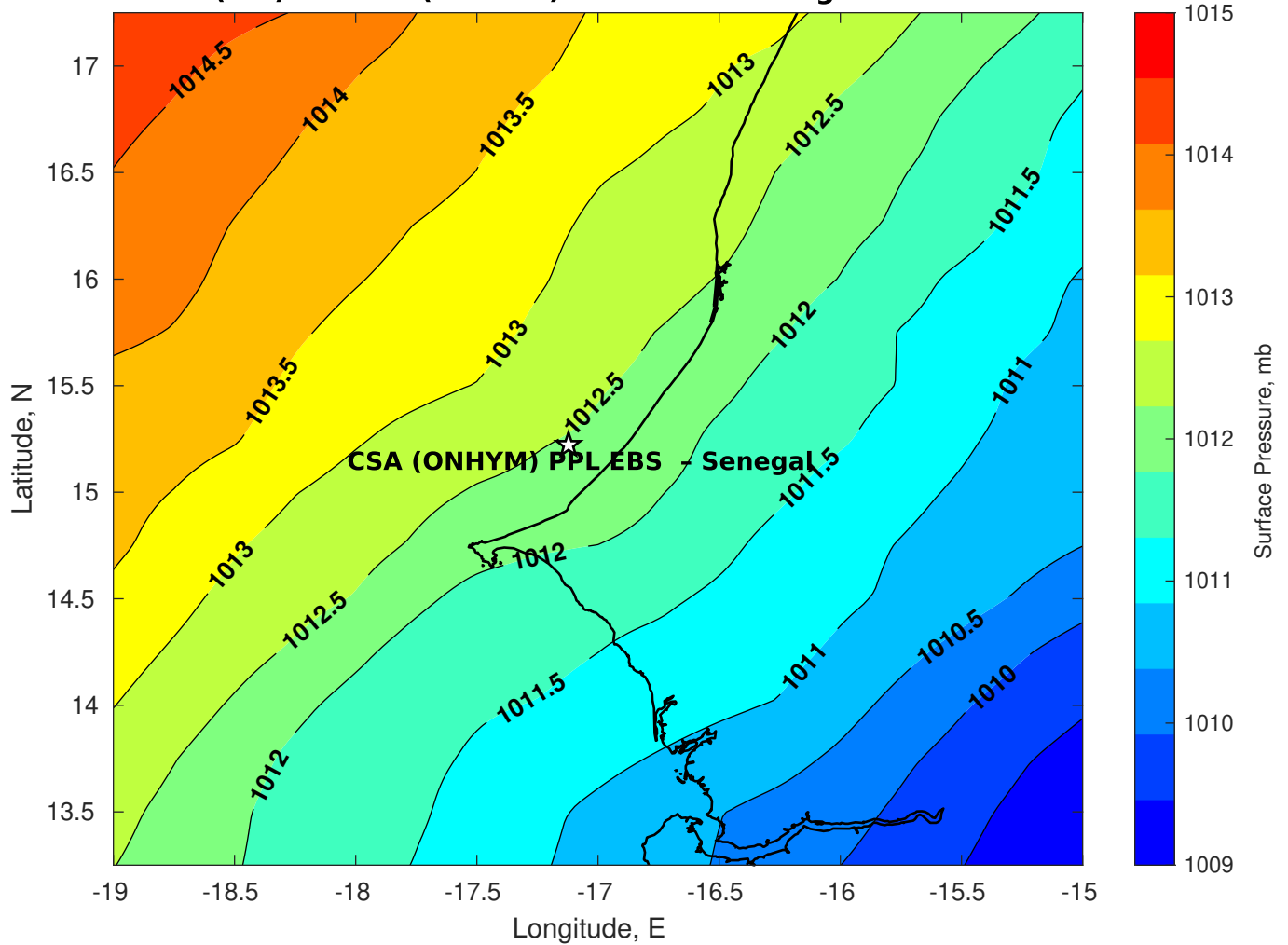
Surface Pressure (mb) for CSA (ONHYM) PPL EBS - Senegal at 27-Mar-2025 00:00:00
