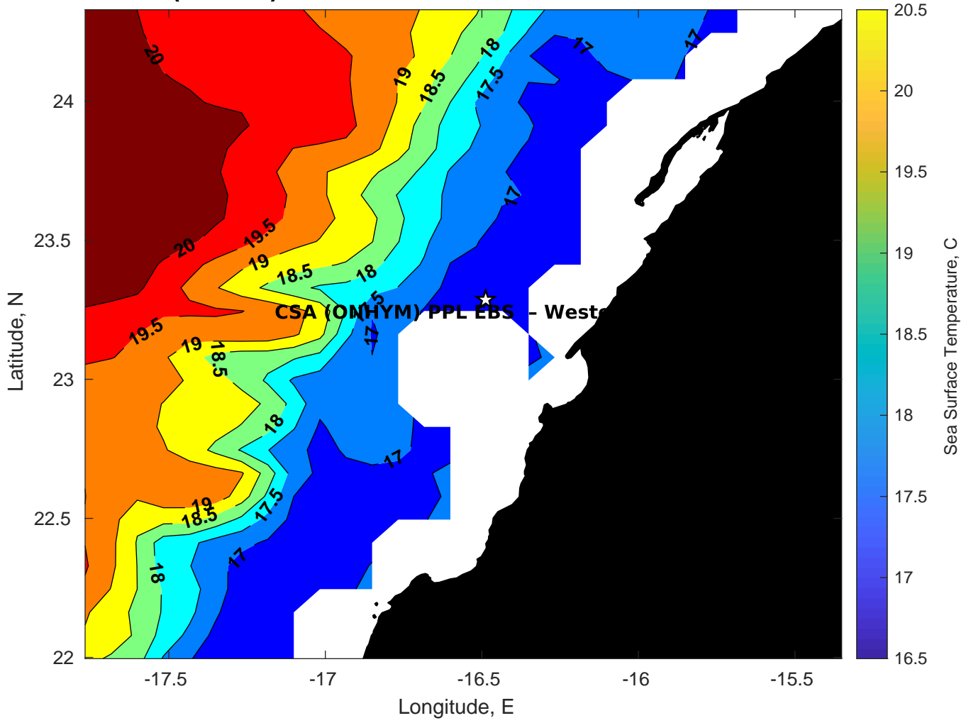
SST for CSA (ONHYM) PPL EBS - Western Sahara at 26-Mar-2025 00:00:00
