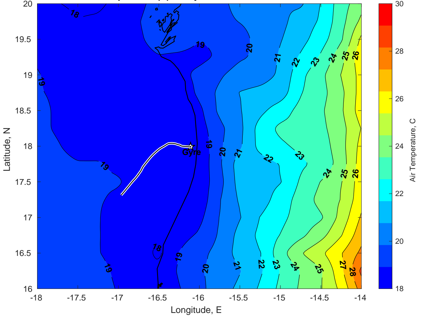
Air Temperature (C) for Gyre at 27-Mar-2025
