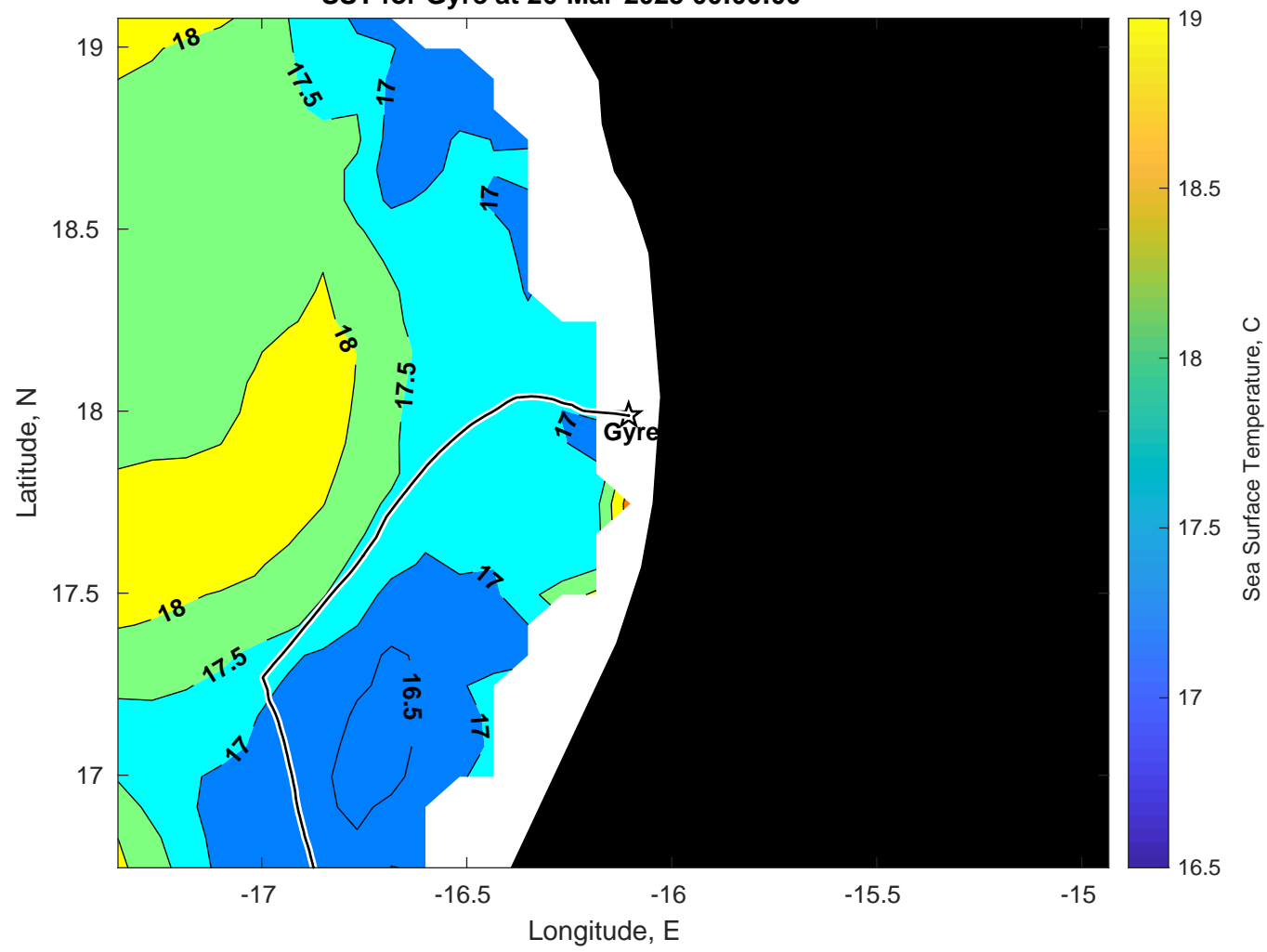
SST for Gyre at 26-Mar-2025 00:00:00
