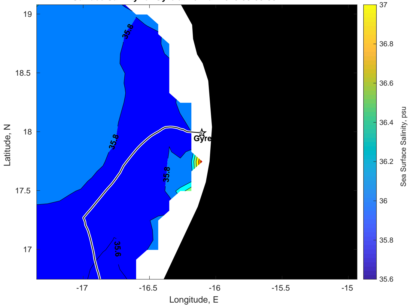
Surface Salinity for Gyre at 26-Mar-2025 00:00:00
