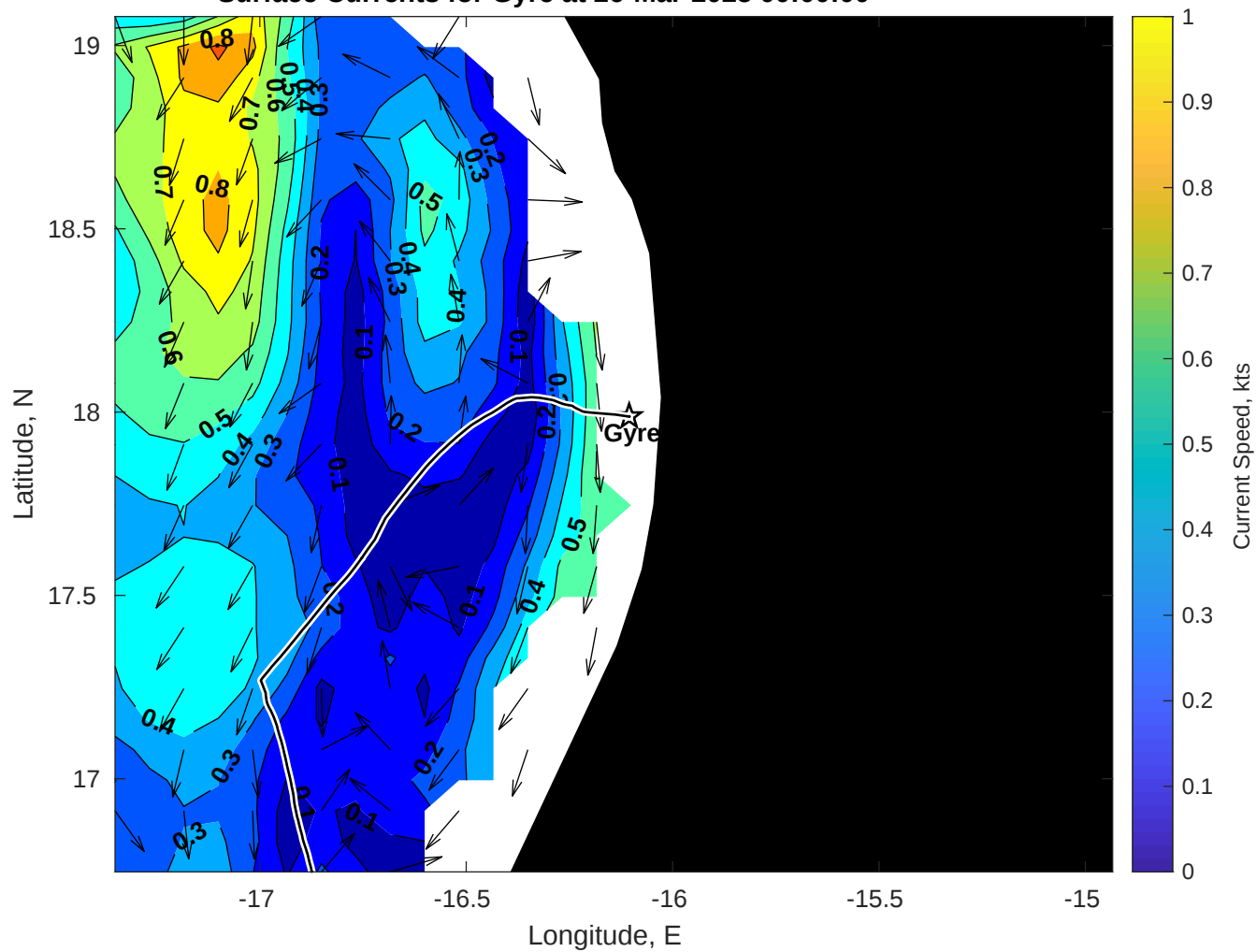
Surface Currents for Gyre at 26-Mar-2025 00:00:00
