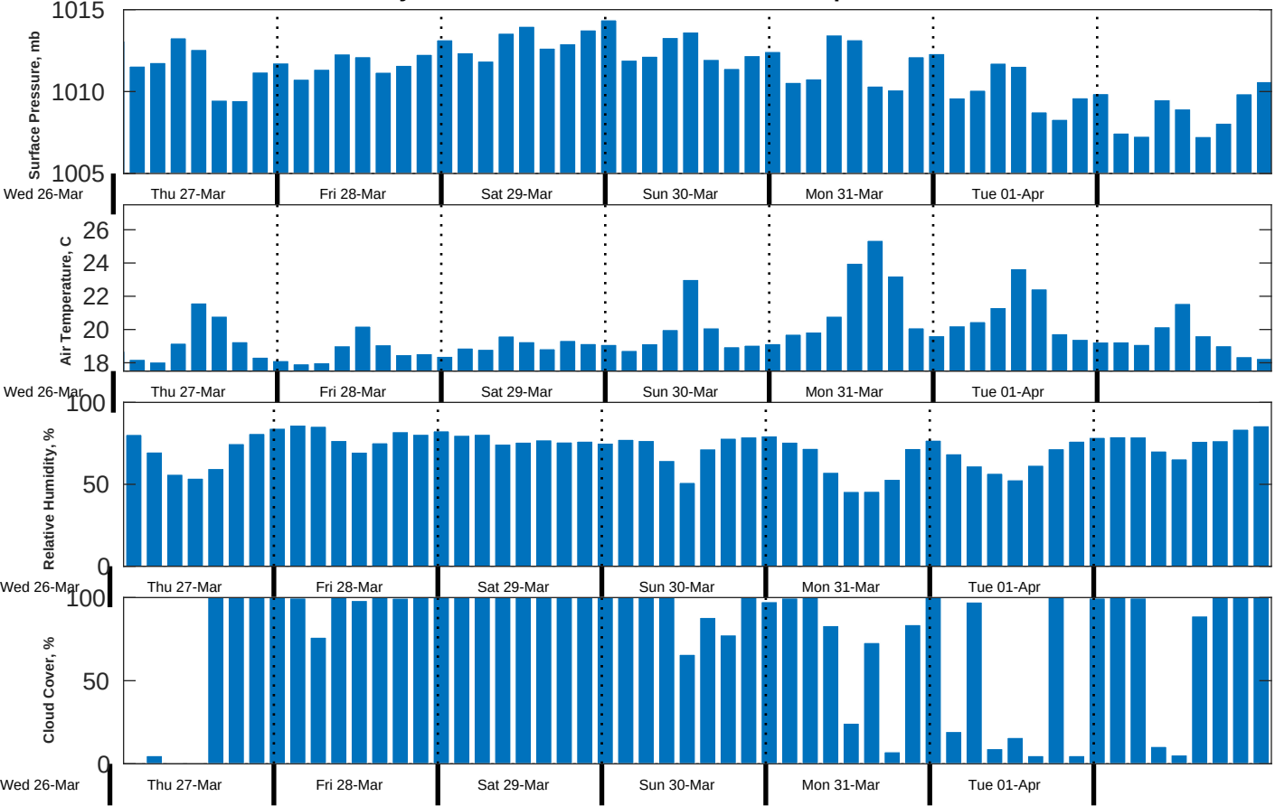
Met Forecast for Gyre from 26-Mar-2025 23:00:00 to 02-Apr-2025 23:00:00
