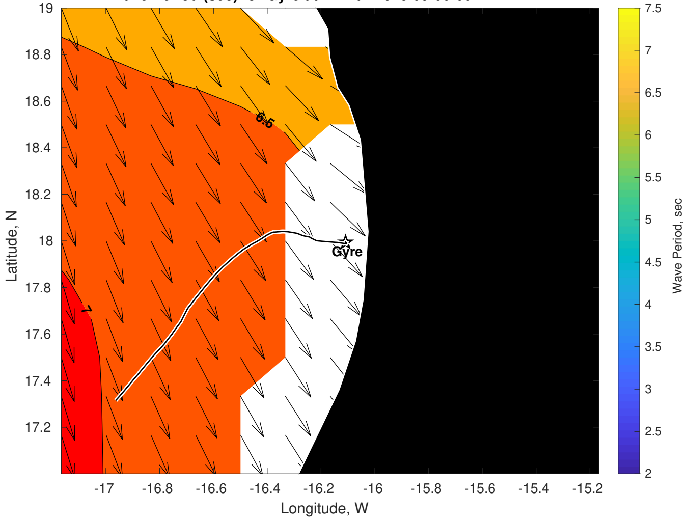
Wave Period (sec) for Gyre at 27-Mar-2025 09:00:00
