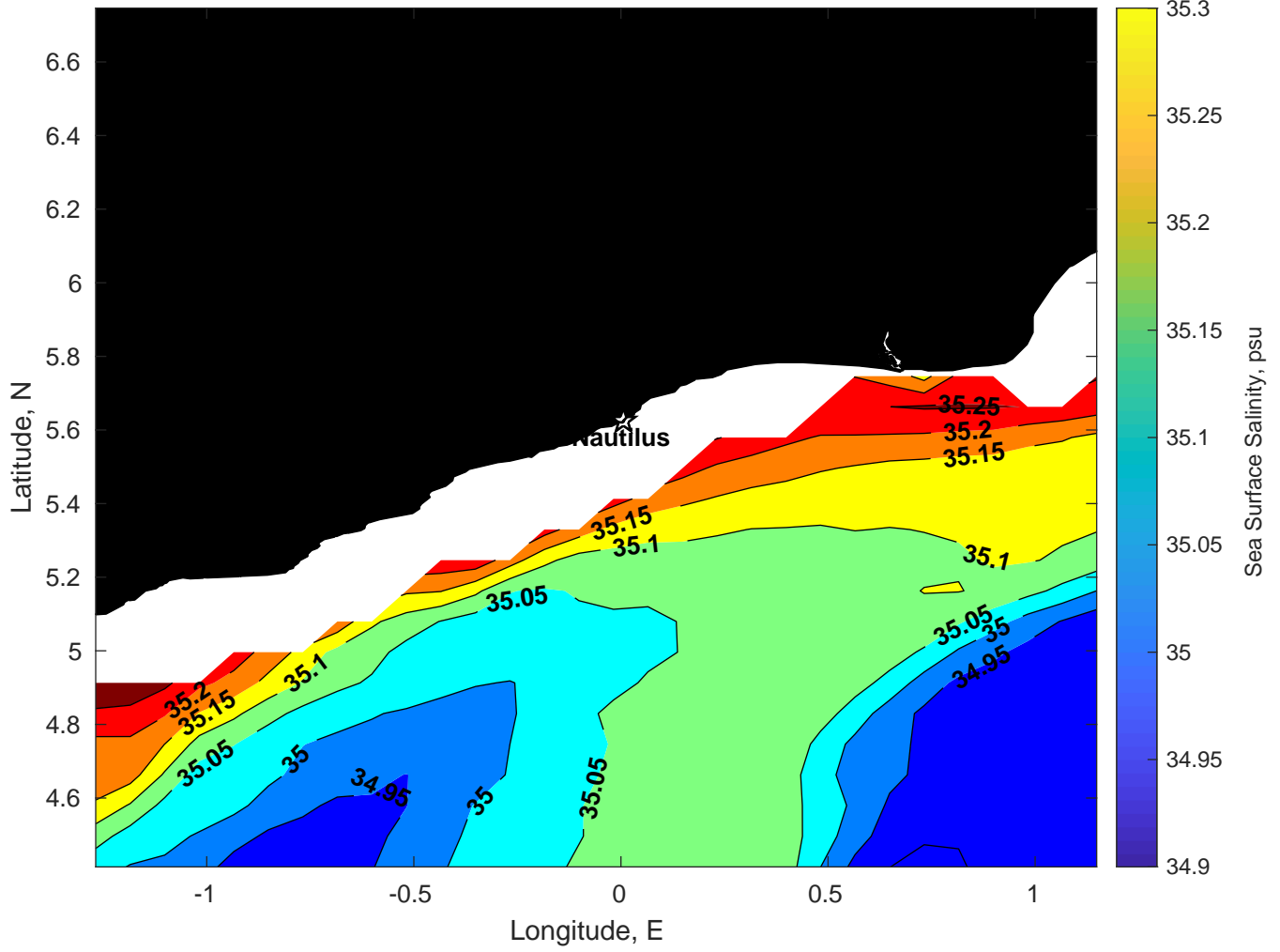
Surface Salinity for Nautilus at 26-Mar-2025 00:00:00
