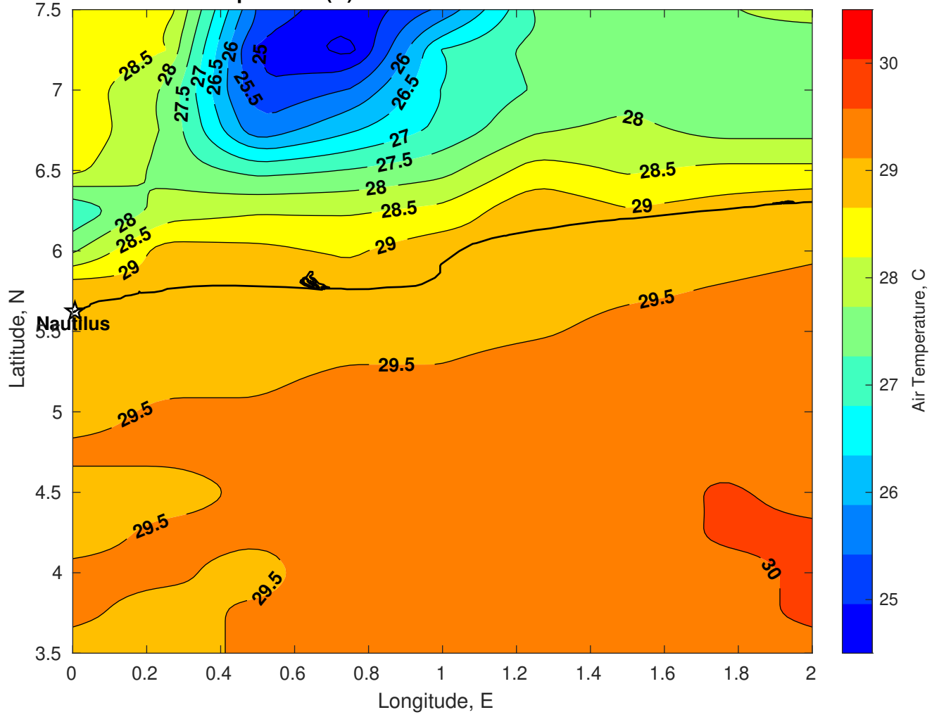
Air Temperature (C) for Nautilus at 27-Mar-2025
