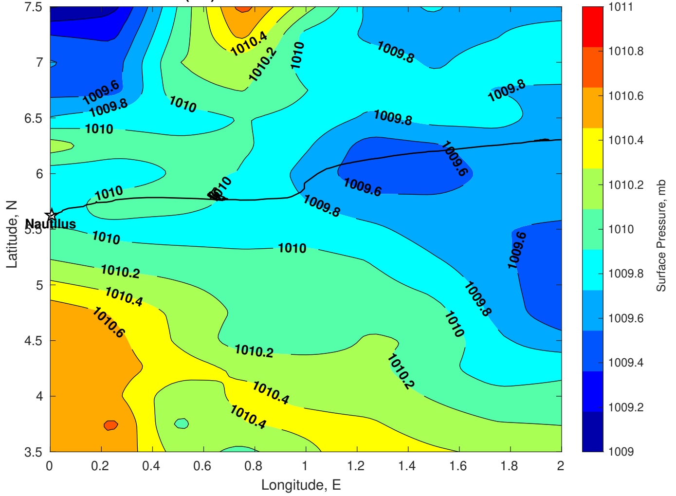
Surface Pressure (mb) for Nautilus at 27-Mar-2025 00:00:00
