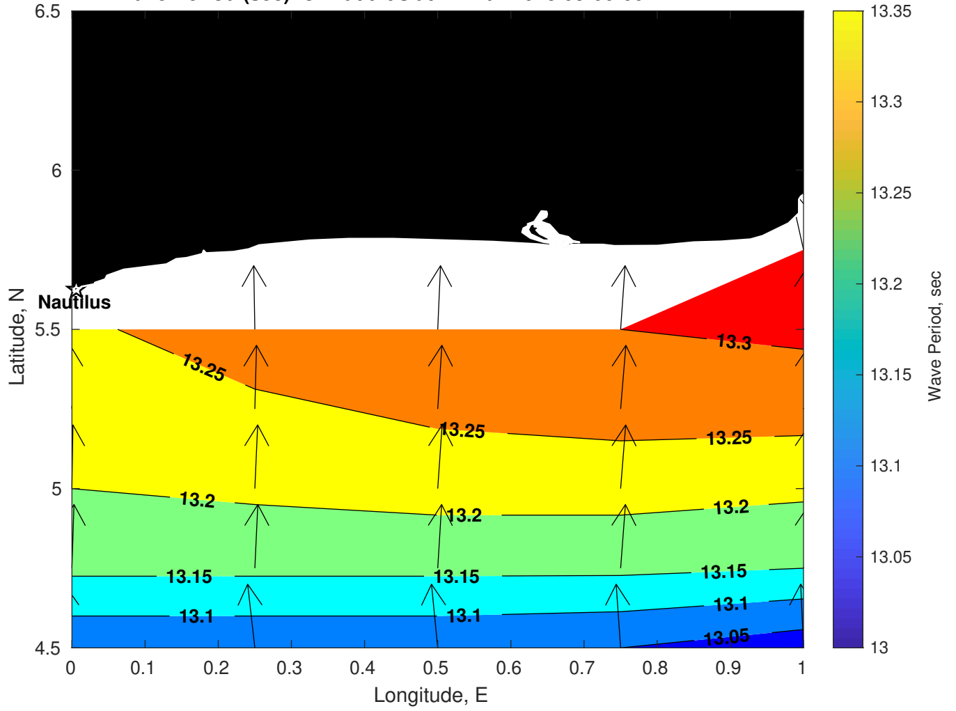
Wave Period (sec) for Nautilus at 27-Mar-2025 09:00:00
