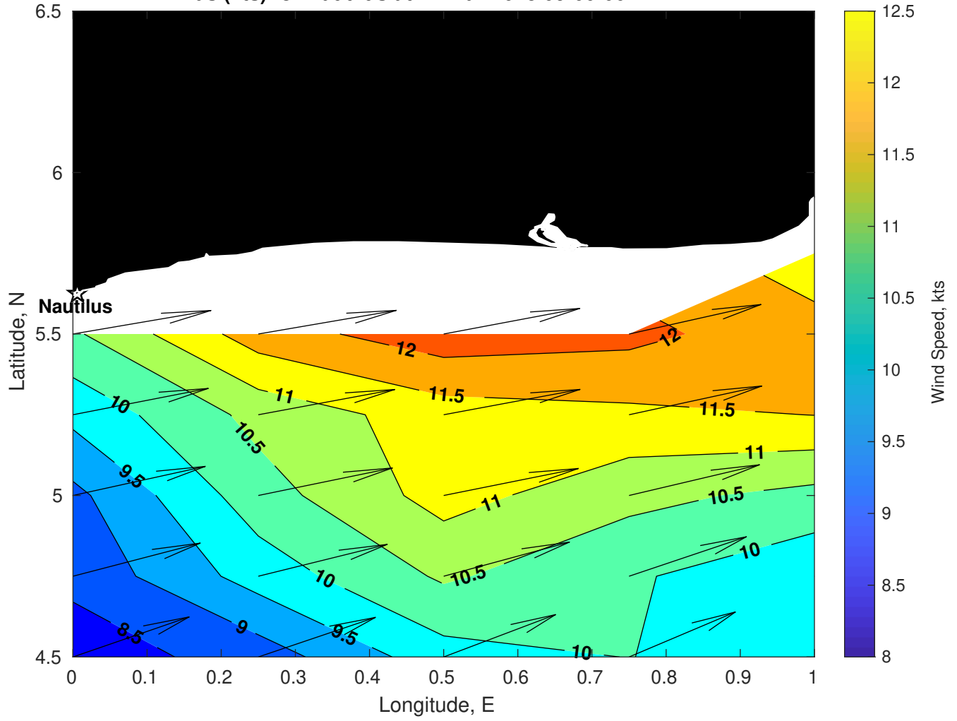
Winds (kts) for Nautilus at 27-Mar-2025 09:00:00
