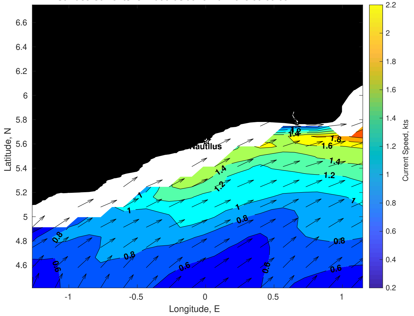
Surface Currents for Nautilus at 26-Mar-2025 00:00:00
