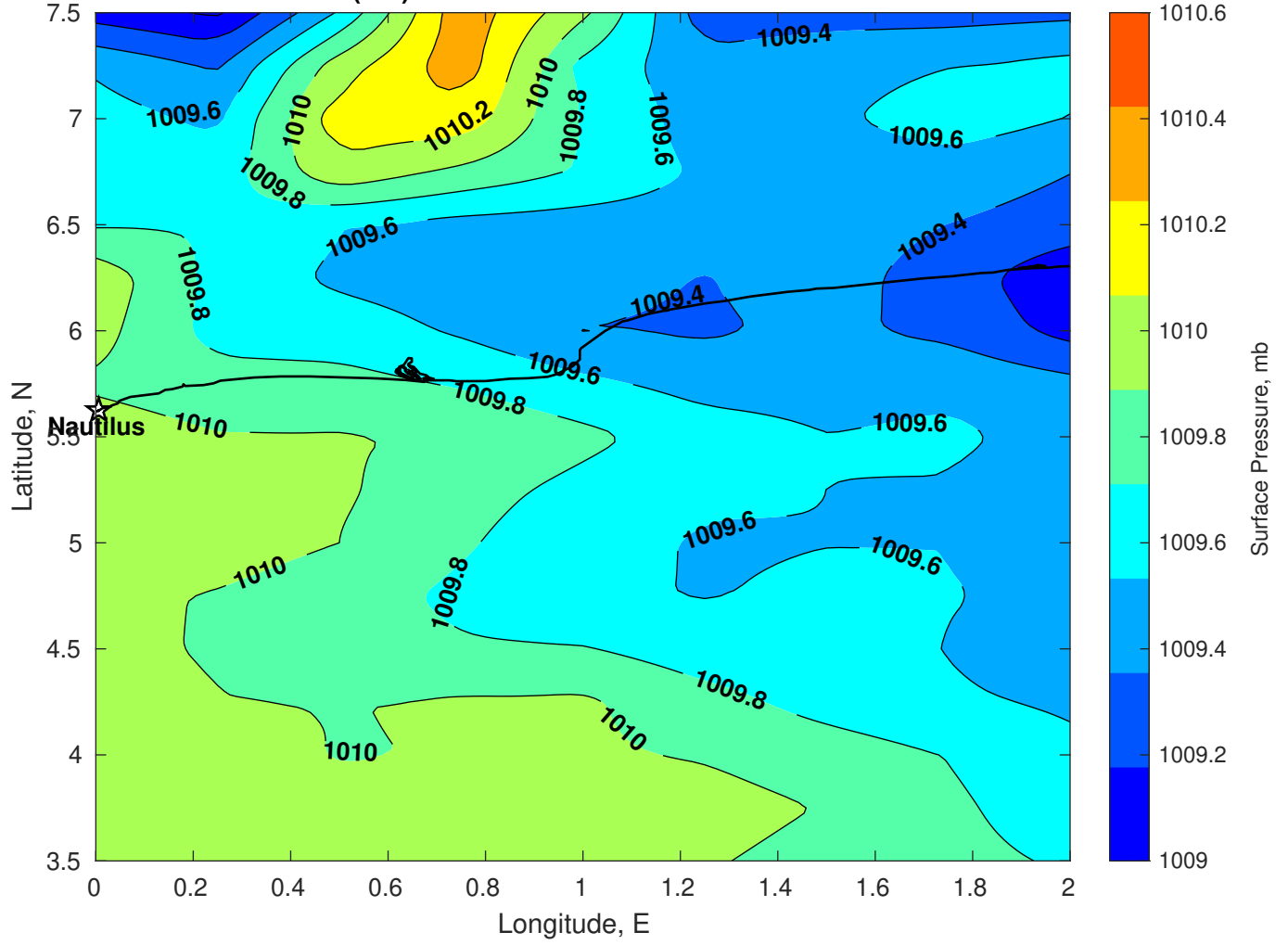
Surface Pressure (mb) for Nautilus at 29-Mar-2025 00:00:00
