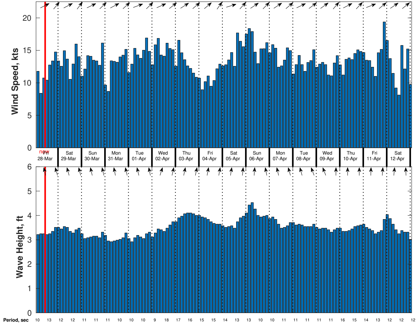
Wind & Wave Forecast for Nautilus from 27-Mar-2025 02:00:00 to 12-Apr-2025 02:00:00
