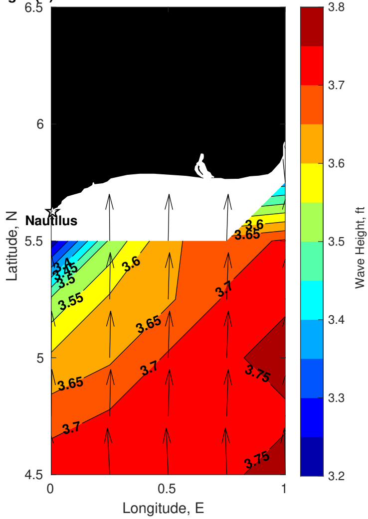
Wave Height (ft) for Nautilus at 27-Mar-2025 09:00:00
