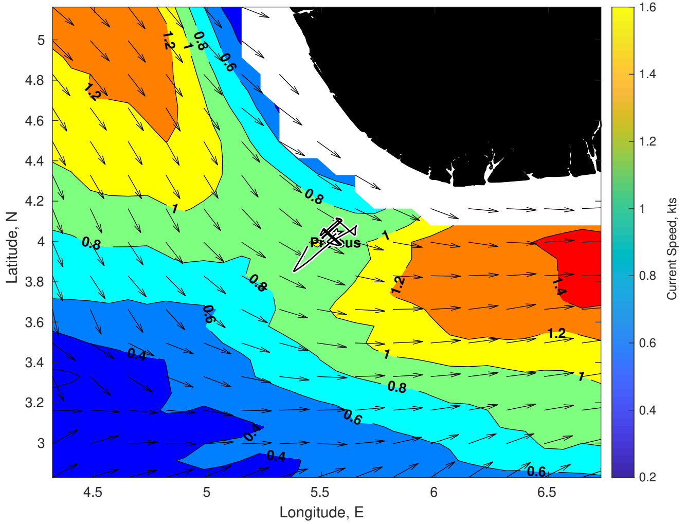
Surface Currents for Proteus at 26-Mar-2025 00:00:00
