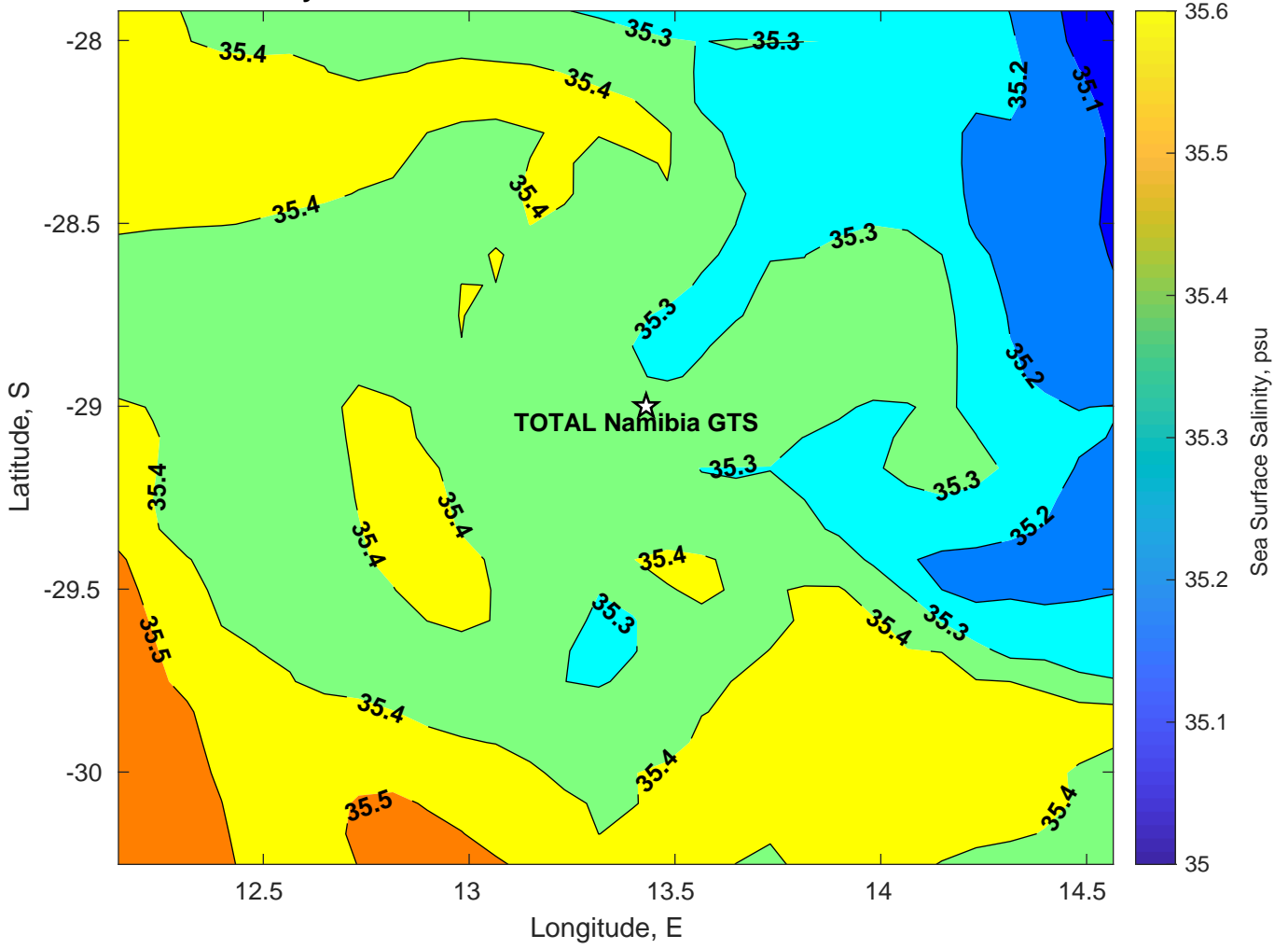
Surface Salinity for TOTAL Namibia GTS at 26-Mar-2025 00:00:00
