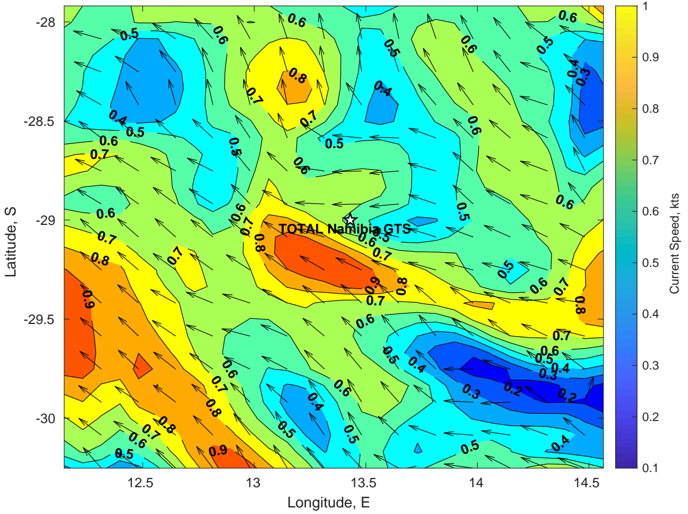
Surface Currents for TOTAL Namibia GTS at 26-Mar-2025 00:00:00
