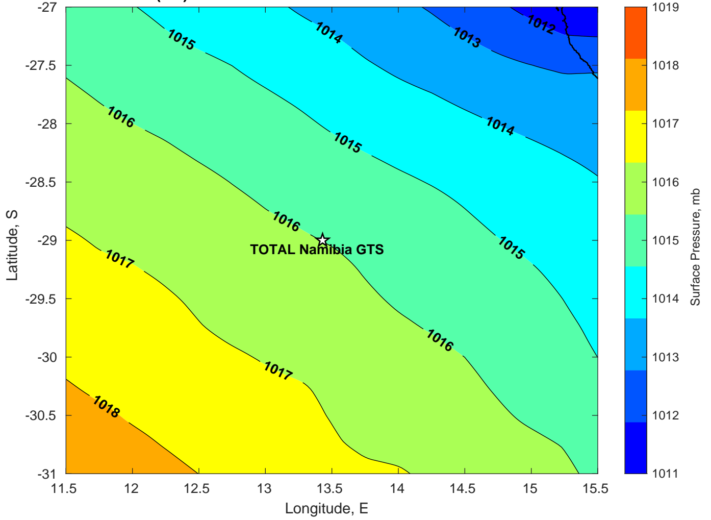
Surface Pressure (mb) for TOTAL Namibia GTS at 27-Mar-2025 00:00:00
