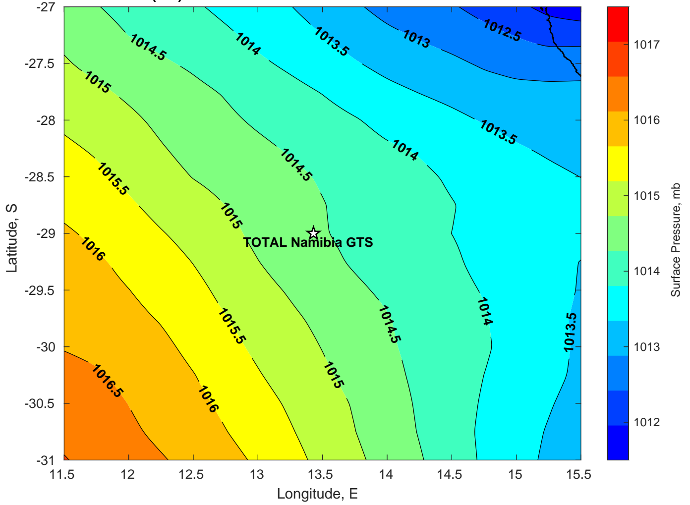
Surface Pressure (mb) for TOTAL Namibia GTS at 28-Mar-2025 00:00:00
