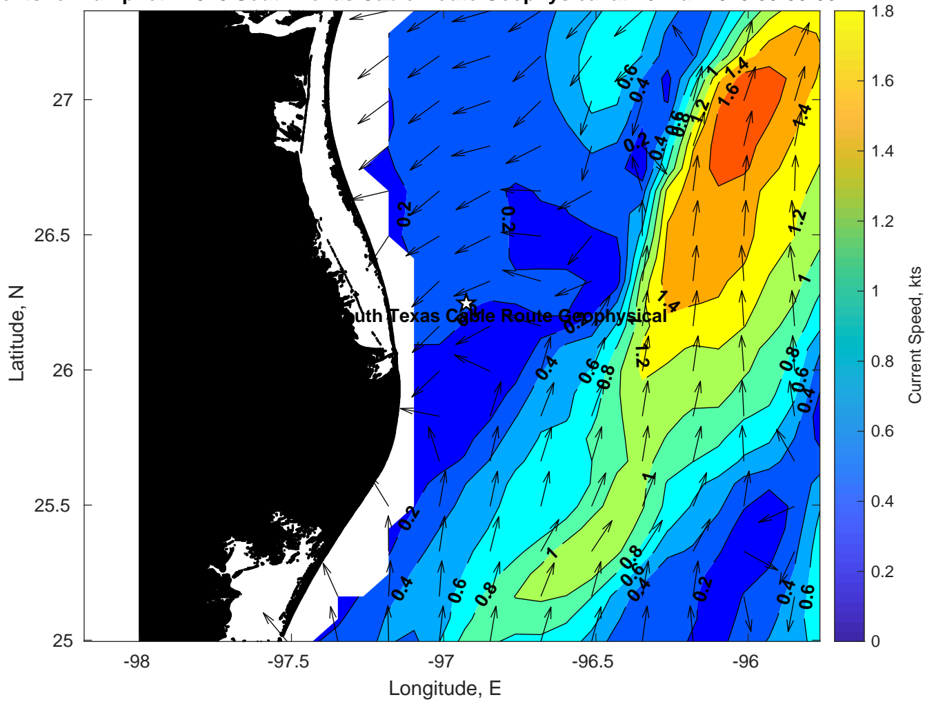
Surface Currents for Tampnet P2378 South Texas Cable Route Geophysical at 26-Mar-2025 00:00:00
