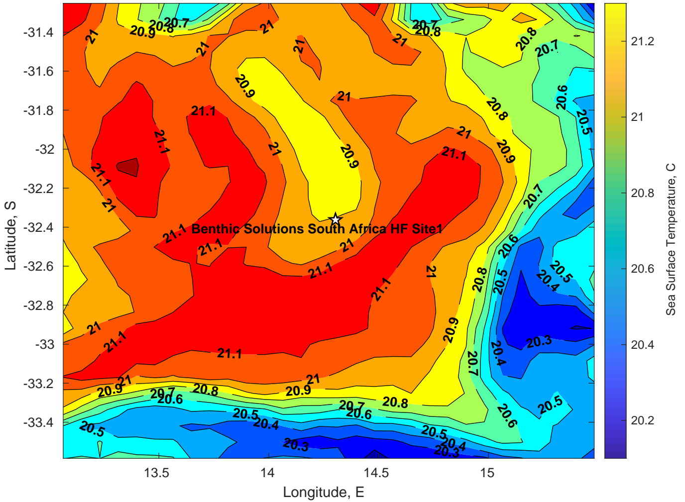
SST for Benthic Solutions South Africa HF Site1 at 27-Mar-2025 00:00:00
