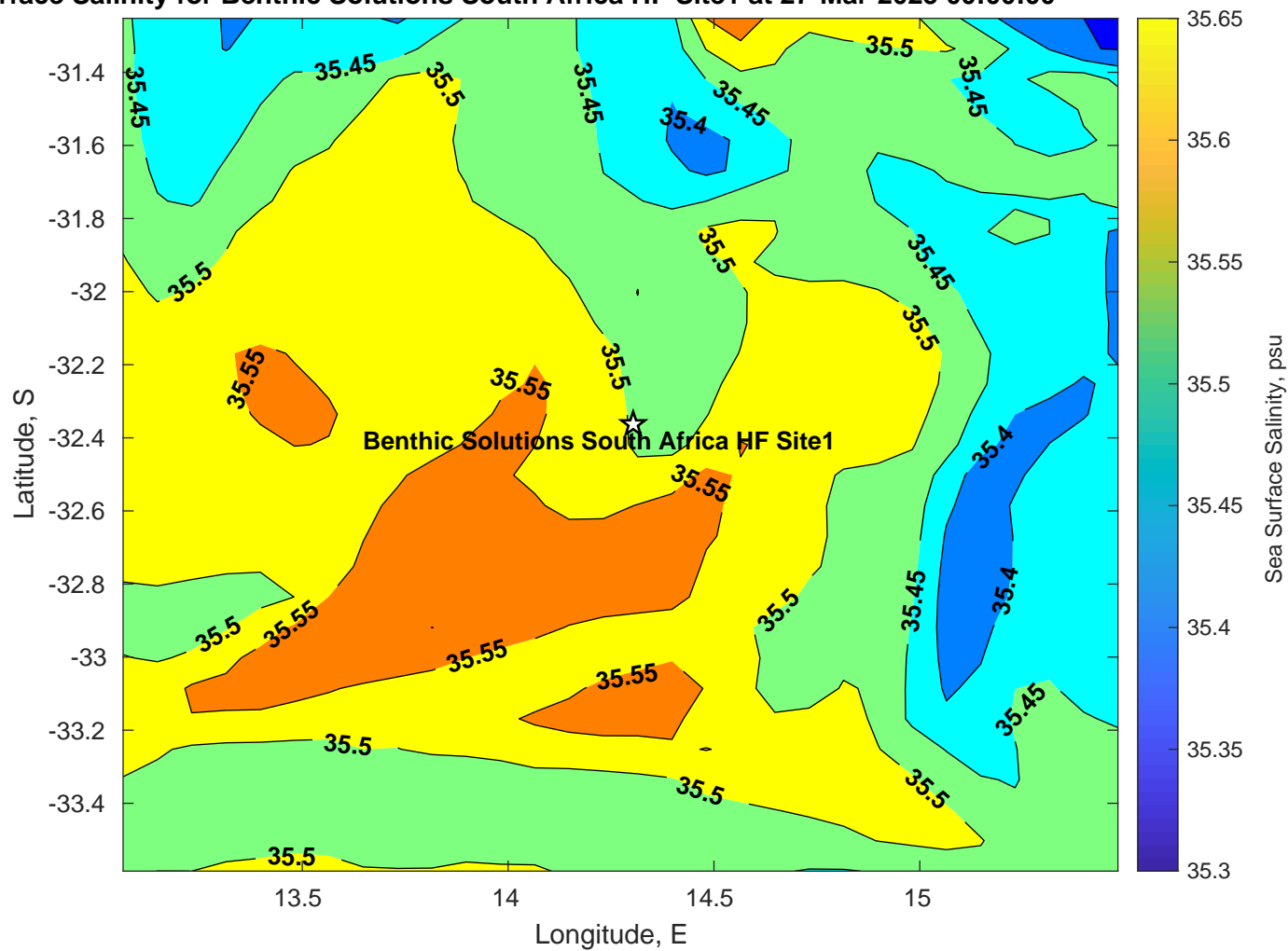
Surface Salinity for Benthic Solutions South Africa HF Site1 at 27-Mar-2025 00:00:00
